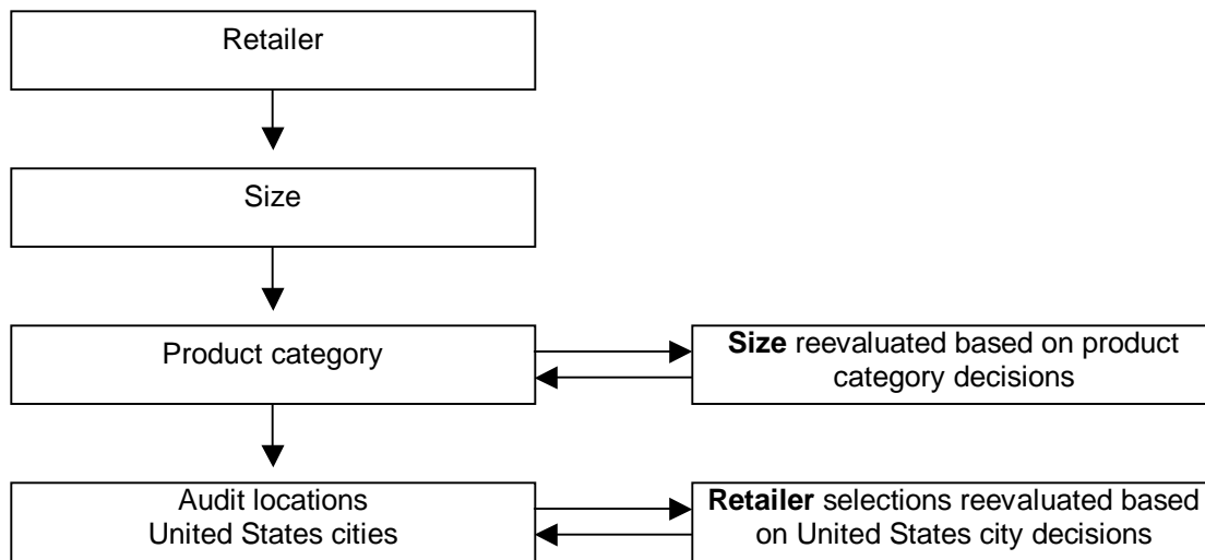
Figure 8: Sample Selection
