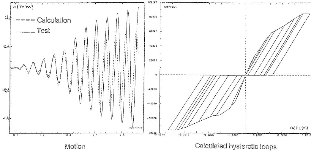
Figure 6 - Response of the wall (frequency of excitation = 26 Hz)
