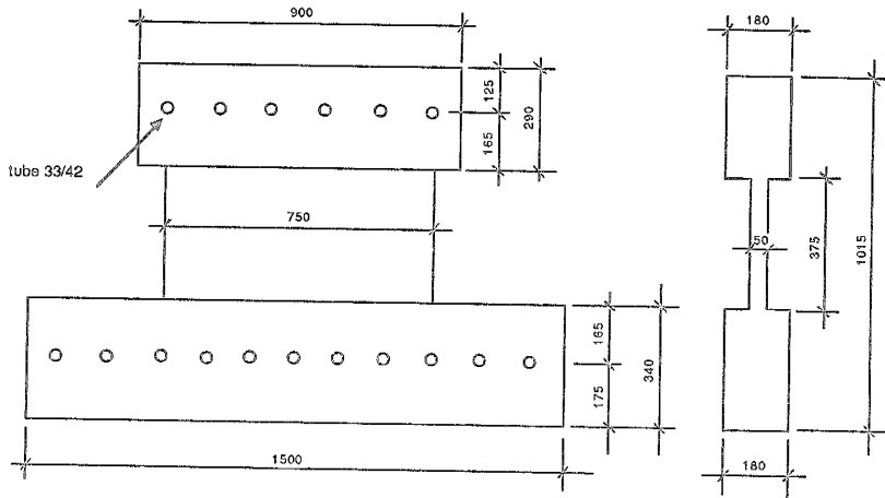
Figure 1 - Geometry of the shear wall (unit = mm)
