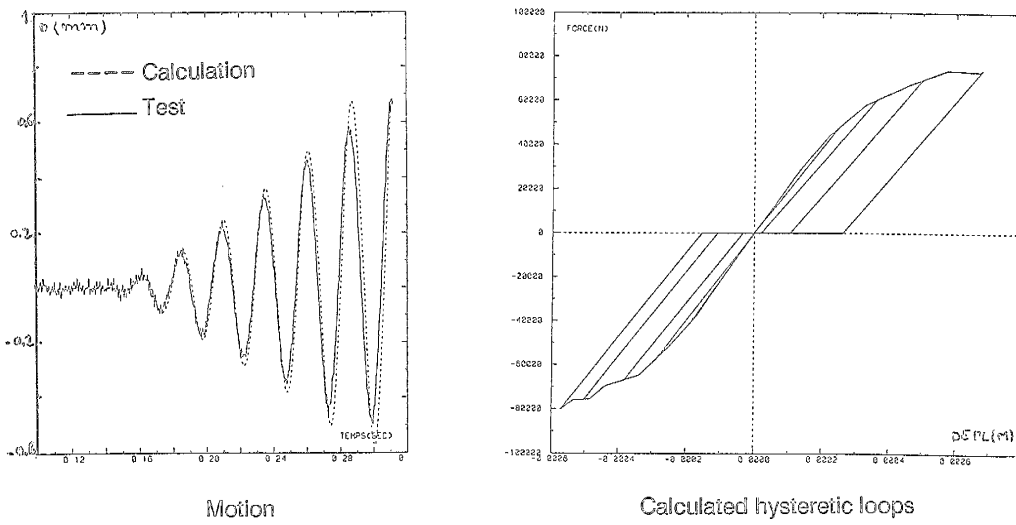
Figure 7 - Response of the wall (frequency of excitation = 40 Hz)
