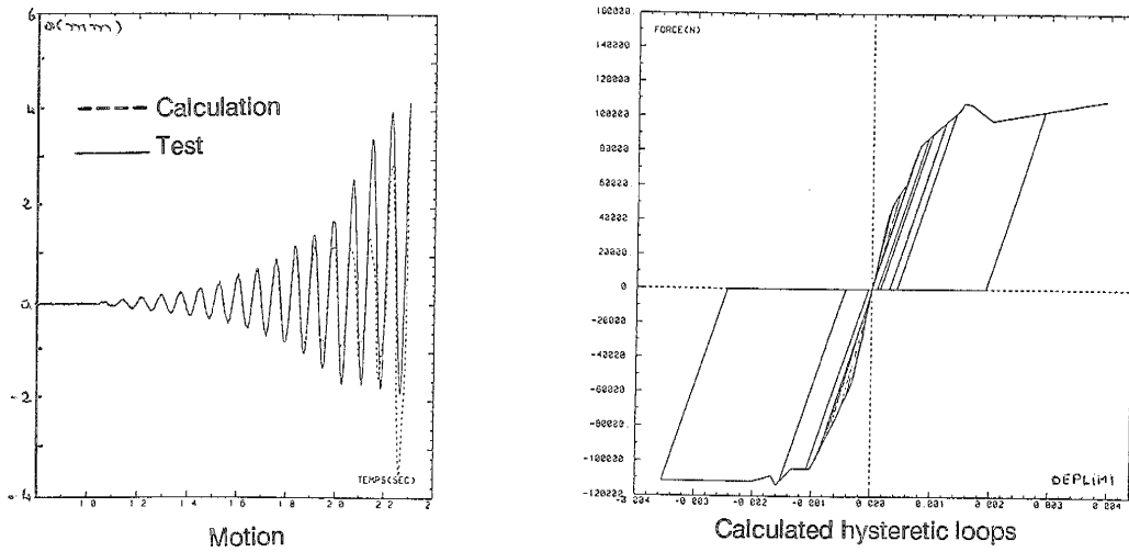
Figure 5 - Response of the wall (frequency of excitation = 13 Hz)
