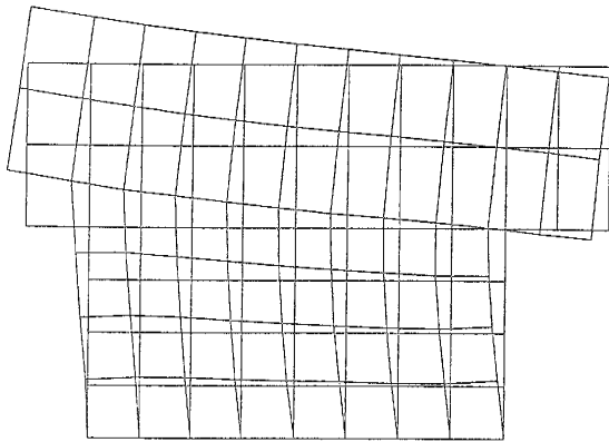
Figure 3 - Second vibration mode frequency = 270 Hz
