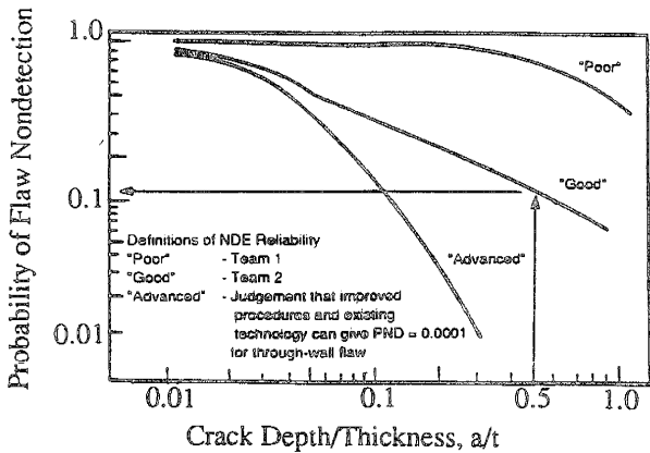
Figure 1. Detection probability of IGSCC in 10 inch stainless steel pipe. (reproduced from reference 2)
