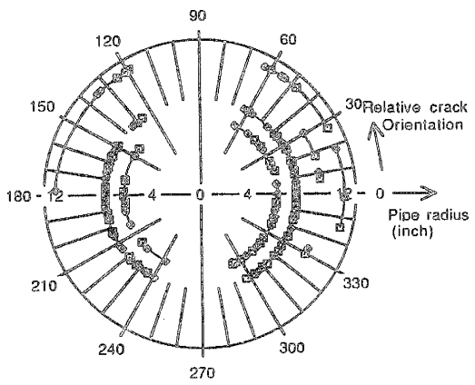
Figure 4. SRS crack angular orientation data.
