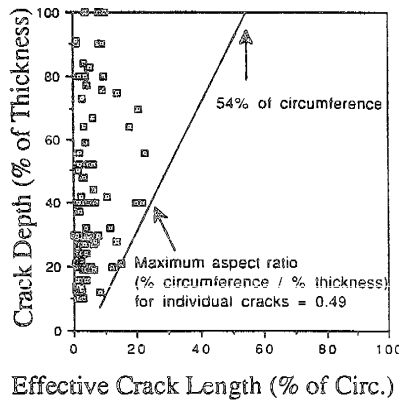
Figure 2. SRS IGSCC shape data.
