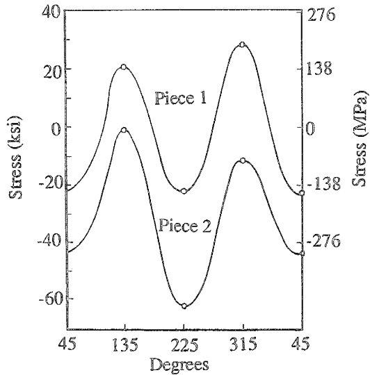
Figure 3. Ten inch pipe inside surface longitudinal residual stress measurements taken 0.1 inch from weld line. (reproduced from reference 3)
