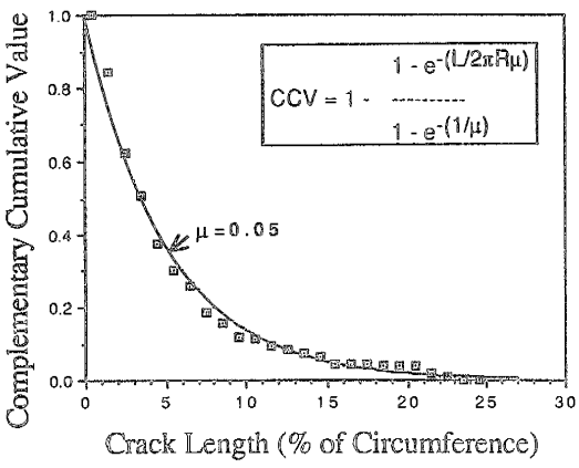
Figure 6. Complementary cumulative distribution for SRS data.
