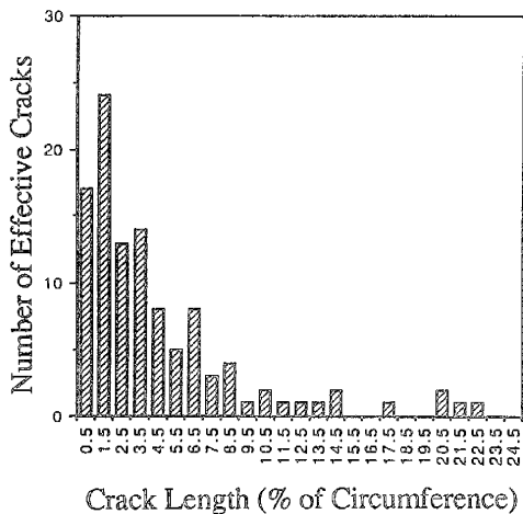
Figure 5. Crack size distribution for IGSCC in SRS primary coolant piping.
