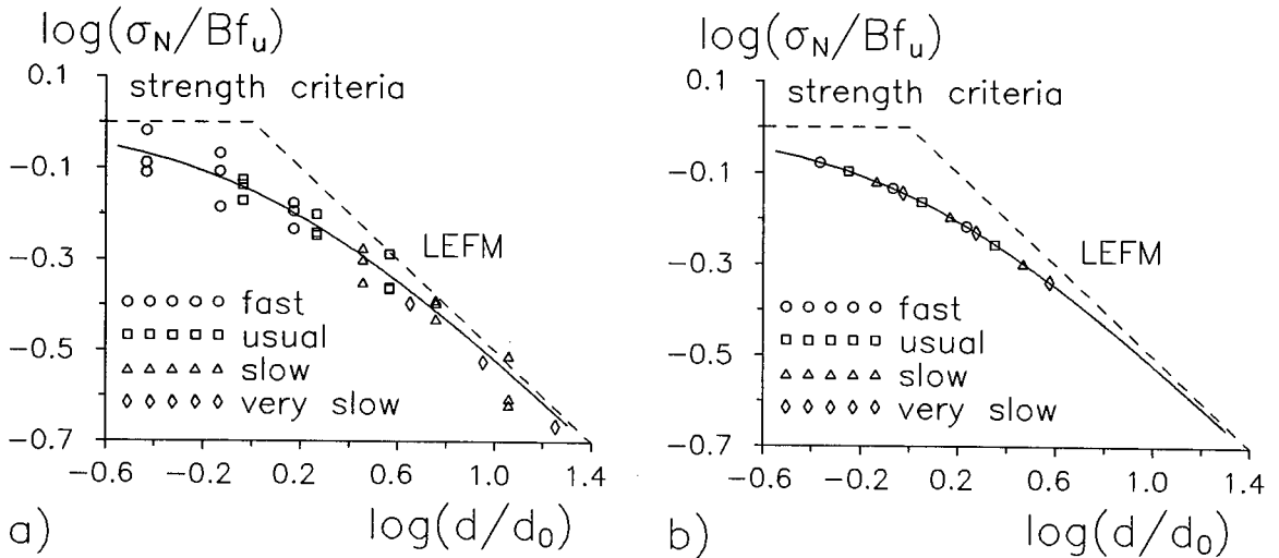
Figure 2: Size effect for concrete: a) experiments, b) theory.
