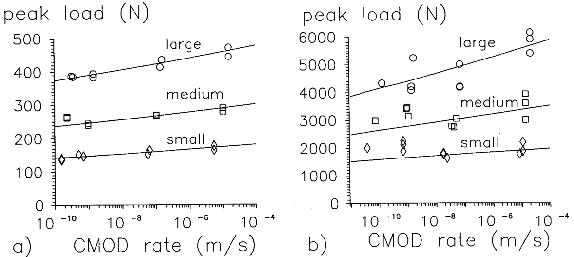
Figure 1: Rate effect for a) limestone, b) concrete.
