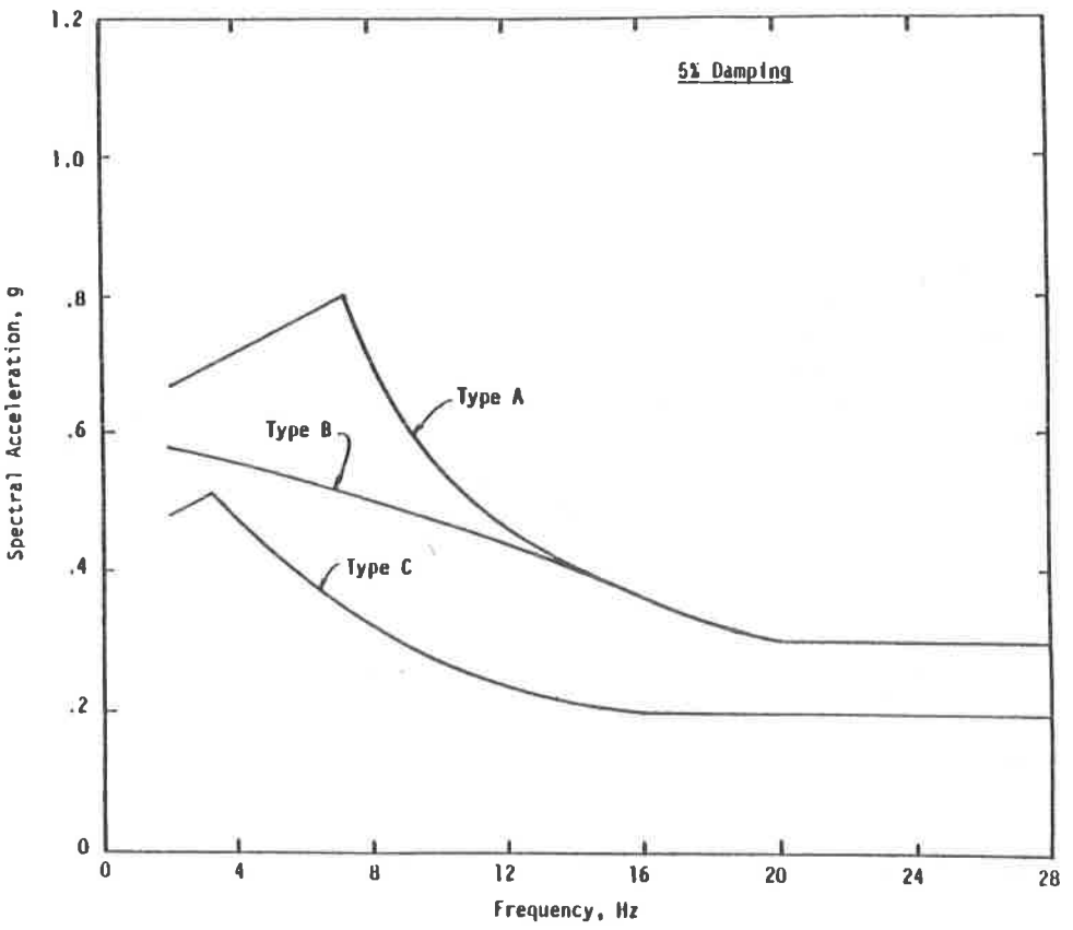
Figure 1. Smoothed Average Horizontal Ground Response Spectra
