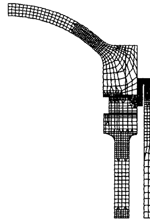
Figure 3 - Finite Element Mesh
