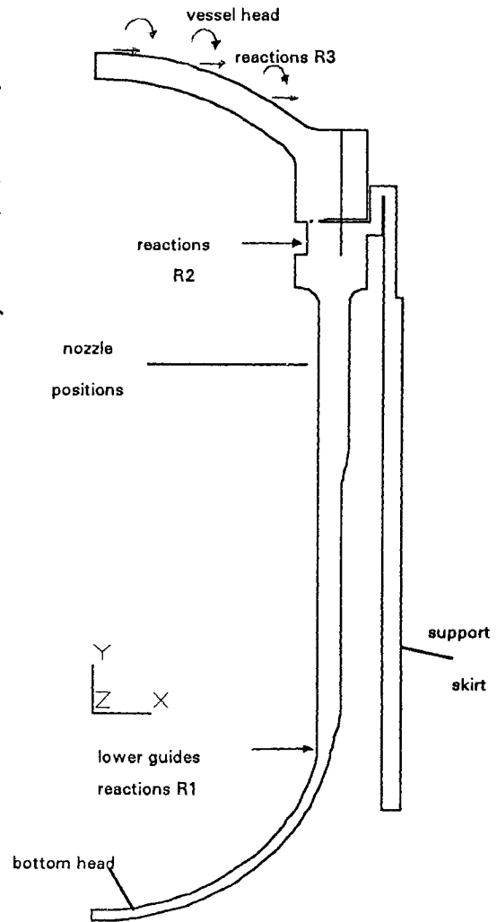
Figure 1 - Vessel
