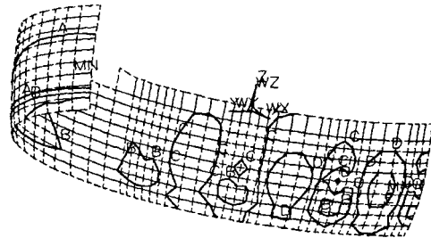
Figure 7 - SI at internal surface - MPa (A = 137; B = 161; C = 184; D = 208; E = 231; MX = 243)
