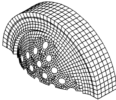
Figure 2.a - Upper head model
