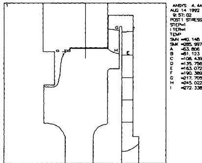
Figure 4 - Temperature distribution (°C)
