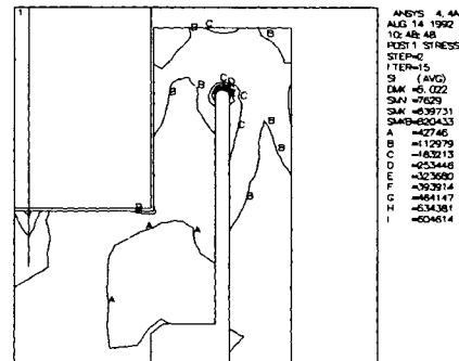
Figure 5 - Stress distribution (Pa)
