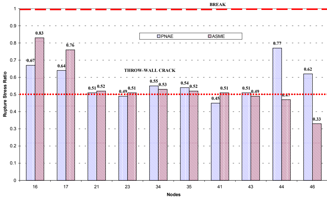
Fig. 6 Comparative PNAE – ASME HELBA Analysis Results
