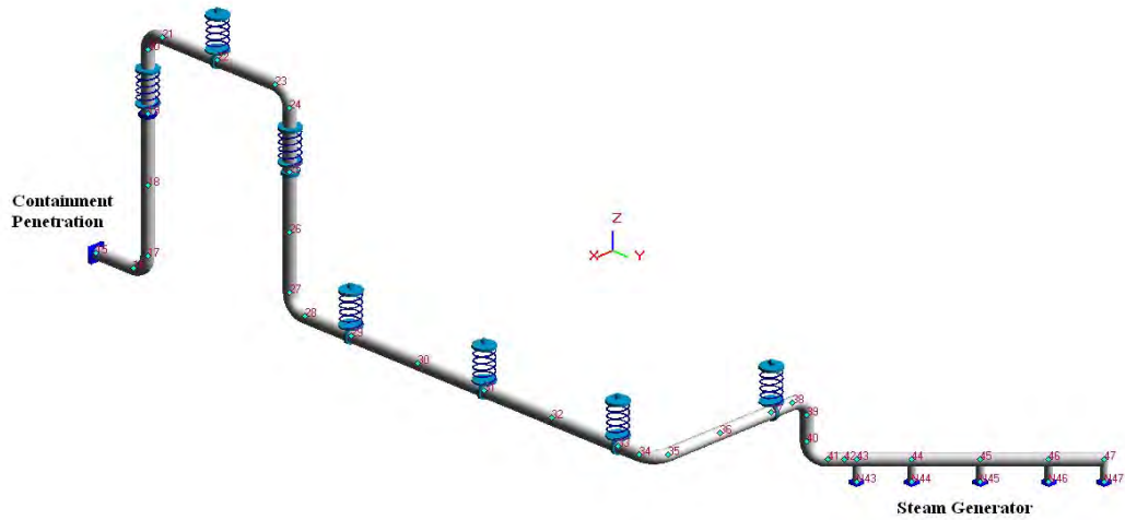
Fig. 4 FE Model of Main Steam Line
