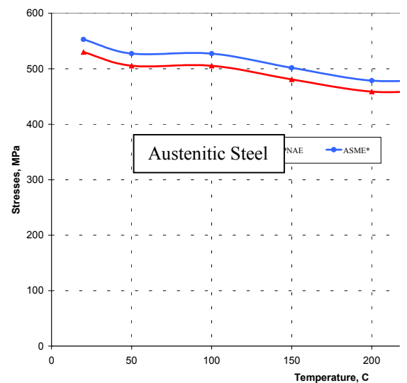
Fig. 2 Comparison of allowable stresses used for determination of rupture location.
