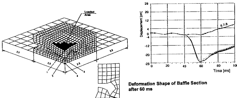
Fig. 8 Mathematical Model and Deformation Shape of the Baffle Element
