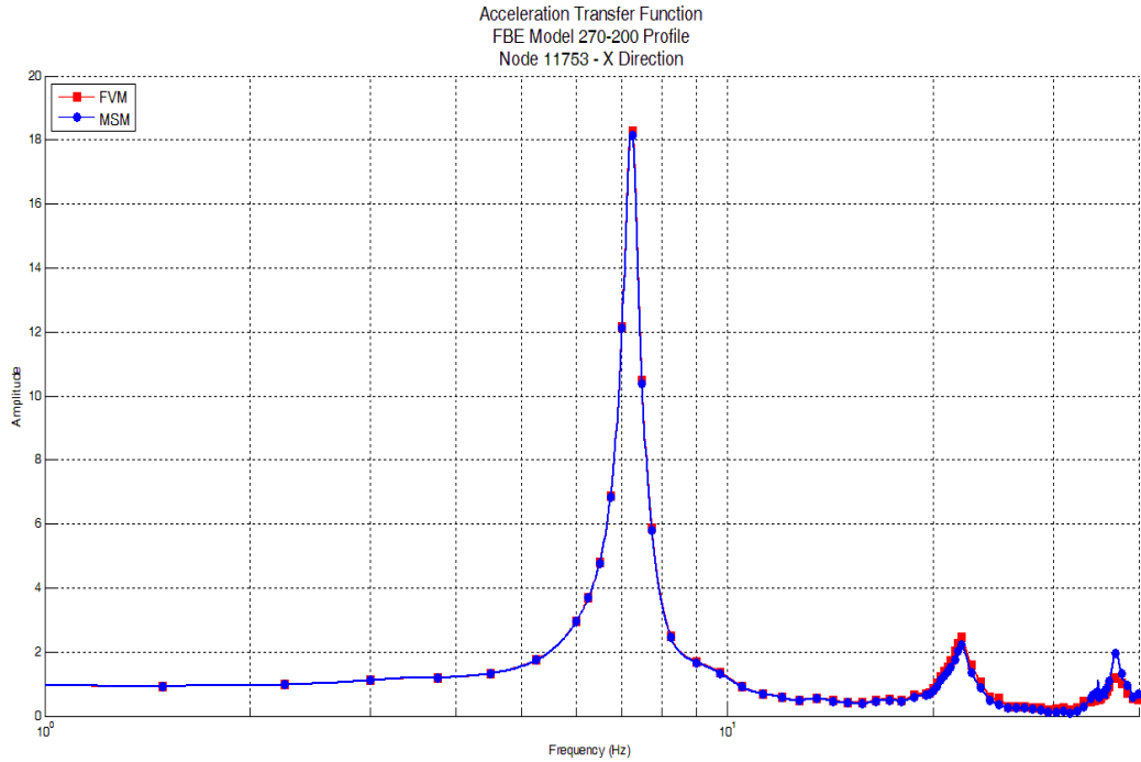
a) ATF Curve
