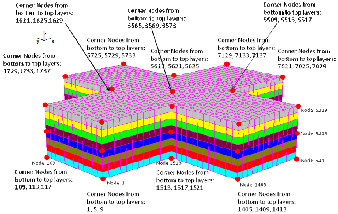
Figure 5 Soil Excavation Model With A Cross-Shape in Horizontal Plane
