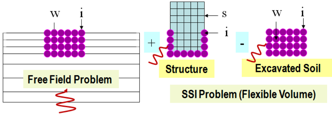
Figure 1. Flexible Volume (FV) Implementation
