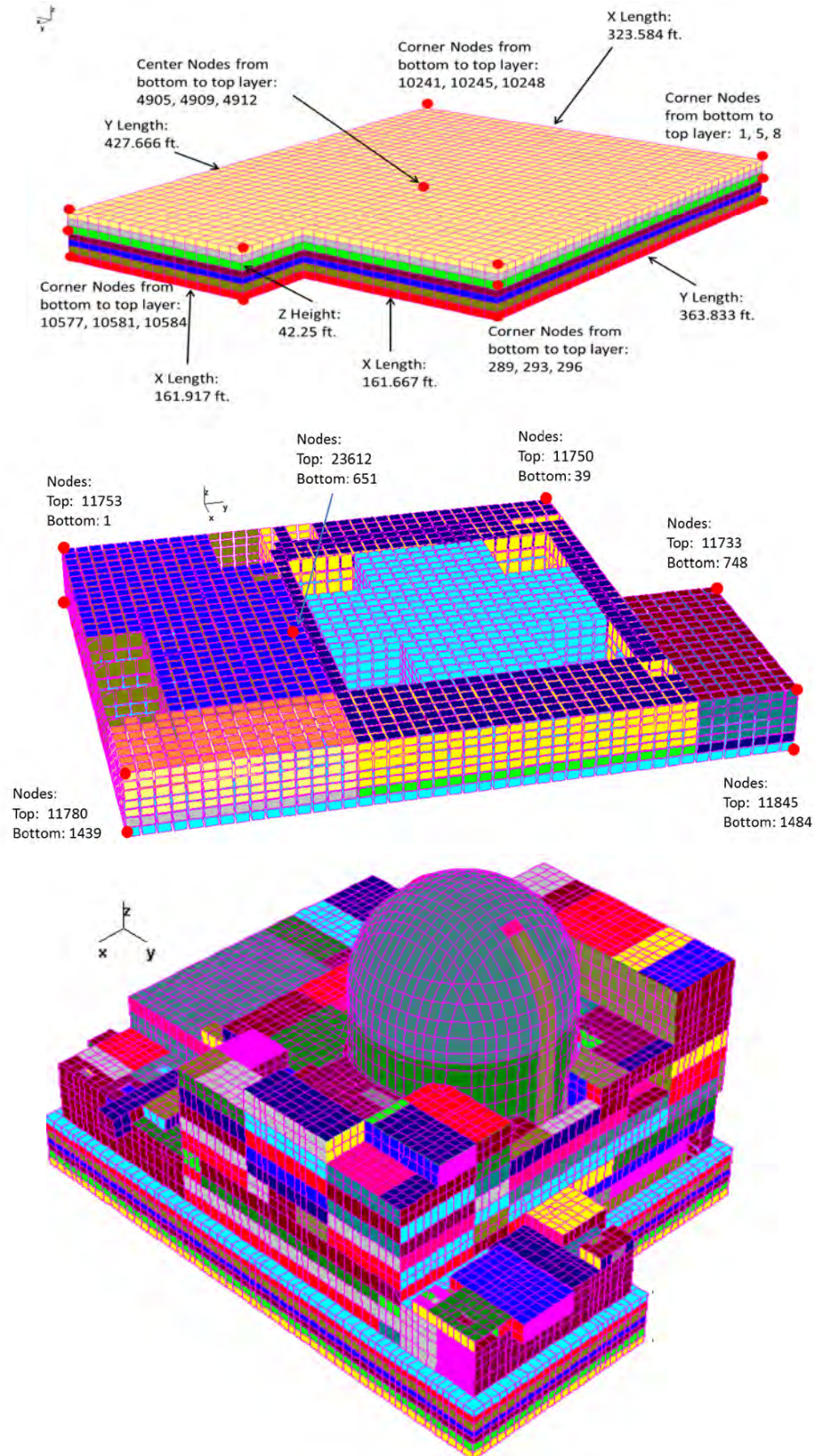
Figure 2 NI Excavation Volume Model (upper), NI Masless Foundation Model (middle) and NI SSI Model including Surrounding Backfill Soil (lower)
