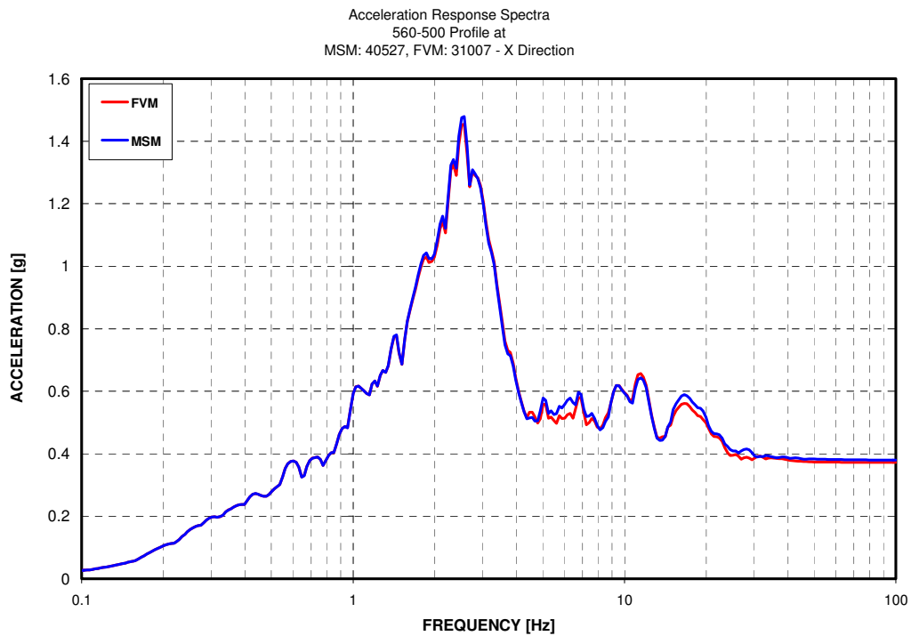
d) 5% Damping ARS
