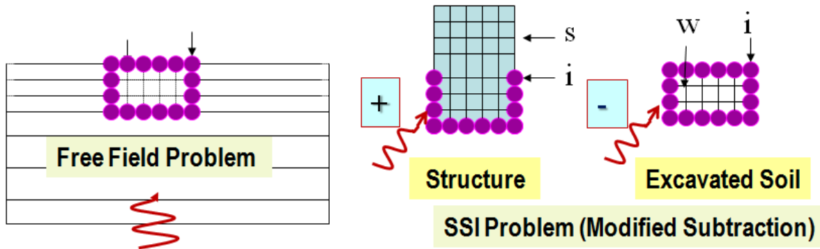
Figure 3. Modified Subtraction Method (MSM) Implementation
