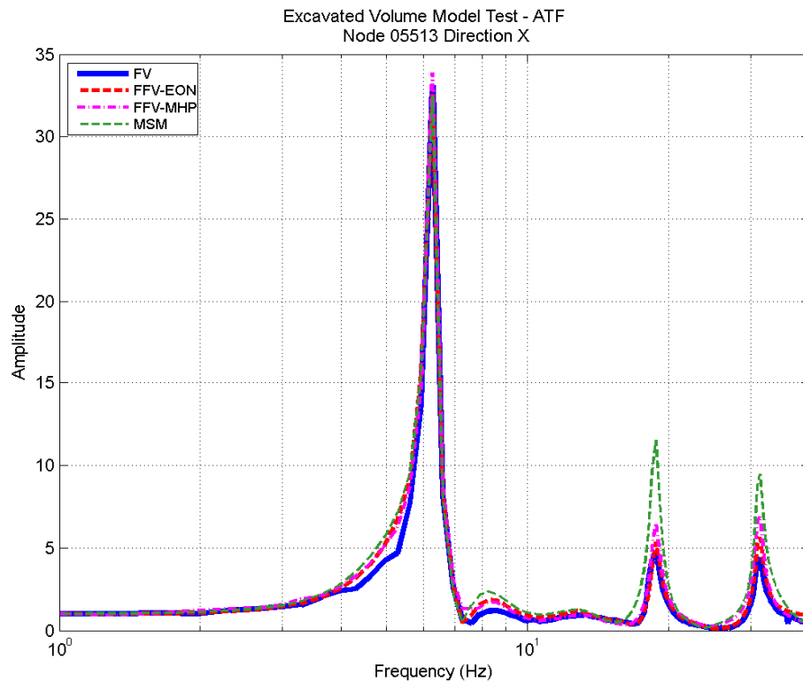
Figure 6 ATF Computed at Interior Corner Middle Level Location (Node 5513 in Figure 4)
