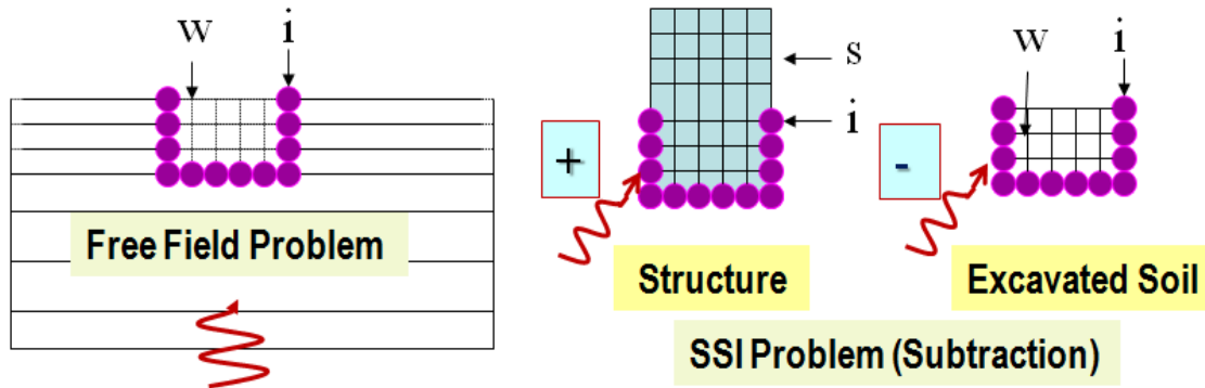
Figure 2. Subtraction Method (SM) Implementation
