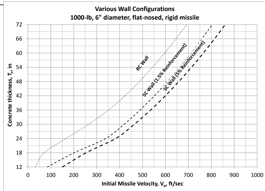
Figure 9 Required Wall Thickness for 1000-lb Missile (Rigid Missile)
