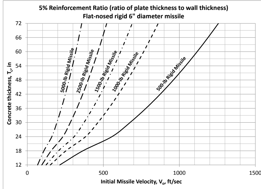
Figure 7 Required SC Wall Thickness to Prevent Perforation (6" Diameter, Flat-Nose, Rigid Missile, 5% Reinforcement)
