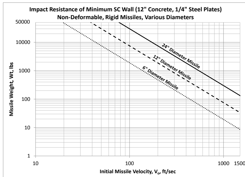
Figure 6 Non-deformable (Rigid) Missile Resistance of Minimum SC Wall ( T_c=12'' ; T_p=0.25'' )
