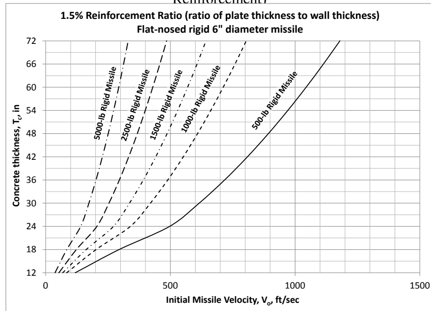
Figure 8 Required SC Wall Thickness to Prevent Perforation (6" Diameter, Flat-Nose, Rigid Missile, 1.5% Reinforcement)
