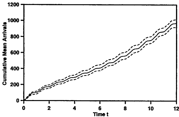
Figure 7: 90% Tolerance Intervals for \mu(t) , t \in [0, 12] , in Case 5
