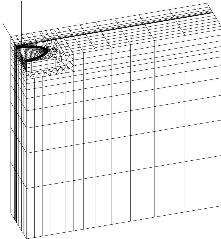
Figure 2: Typical finite element mesh 2a/t = 0.5 , a/c = 0.5 , a/d = 0.375 (23,173 nodes)
