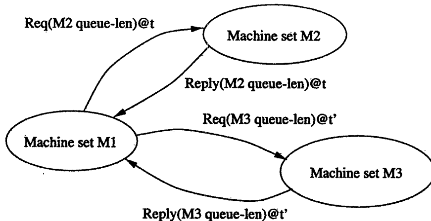
Figure 1: Reading a Remote Variable by Request-Reply Protocol
