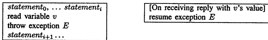
Figure 3: Request-reply approach to read shared variable, using exception mechanism
