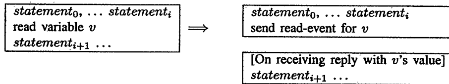
Figure 2: Request-reply approach to read shared variable using manual code partition
