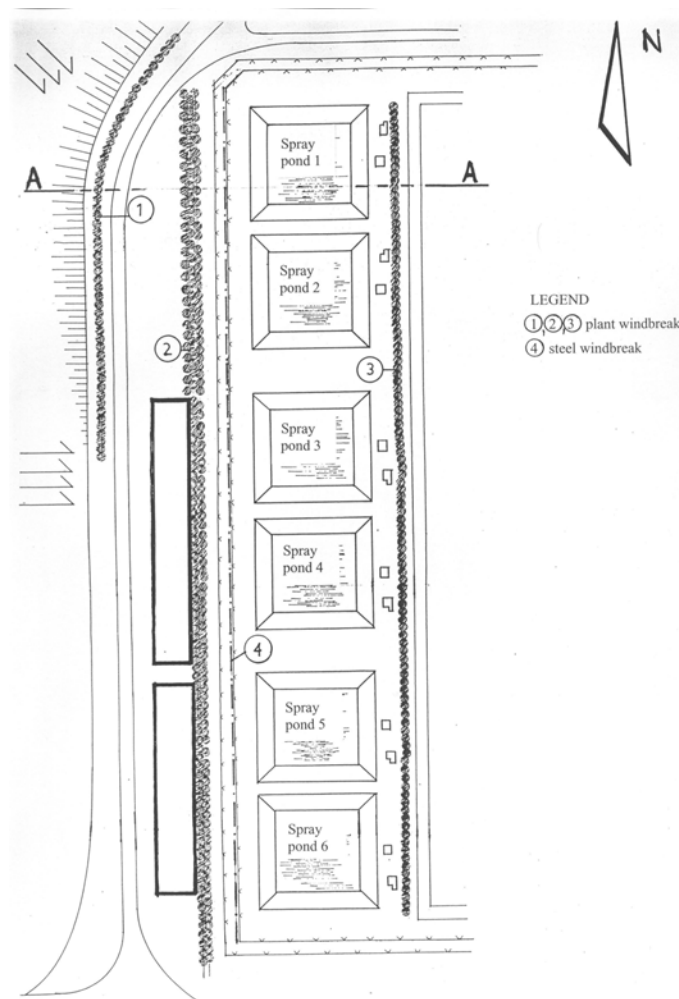
Figure 1 Spray ponds layout. Windbreaks locations
