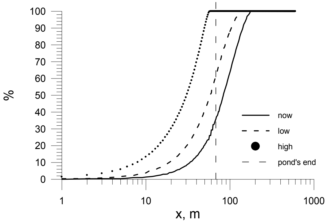
Figure 6 Droplets distribution with a diameter d=100\ \mu\text{m} (the x-axis origin is located at the beginning of the spray pond). (Cases SP12-Now, SP12-PWB-Low, SP12-PWB-High)
