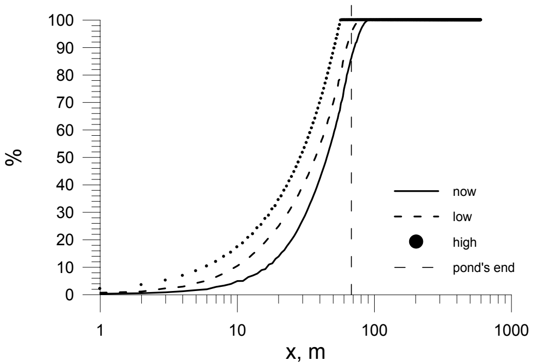
Figure 7 Droplets distribution with a diameter d=250\ \mu\text{m} (the x-axis origin is located at the beginning of the spray pond). (Cases SP12-Now, SP12-PWB-Low, SP12-PWB-High).
