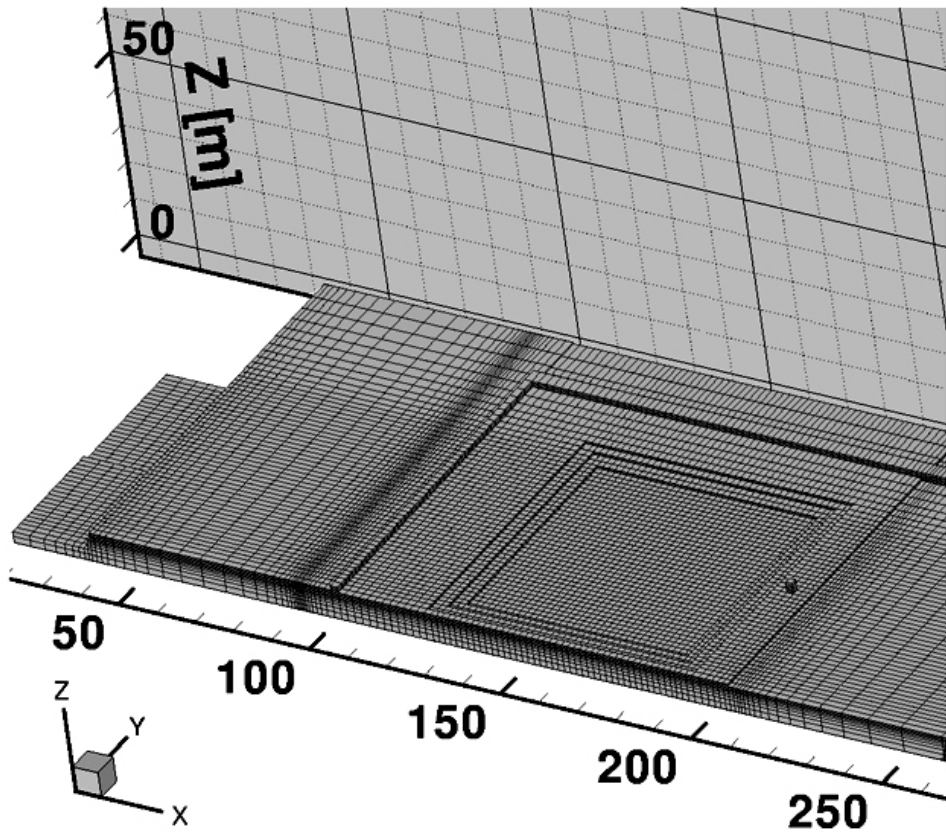
Figure 2 The geometry of the computational domain with the northern spray pond and the numerical grid
