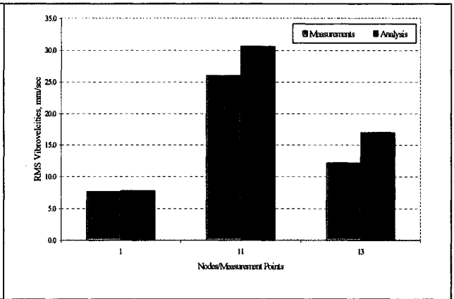
Figure 3. Comparison of Measured and Calculated RMS Value of Vibration for Principal Nodes of the System (1-Valve 1234 Body, 11-Piping 21, 13-Piping 20).
