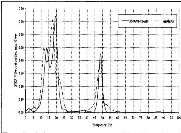
Figure 2. Comparison of Measured Experimentally and Analytical PSD Vibrovelocity (Eigen Value Analysis) for Measurement Point 1 (Valve 1234 Body).
