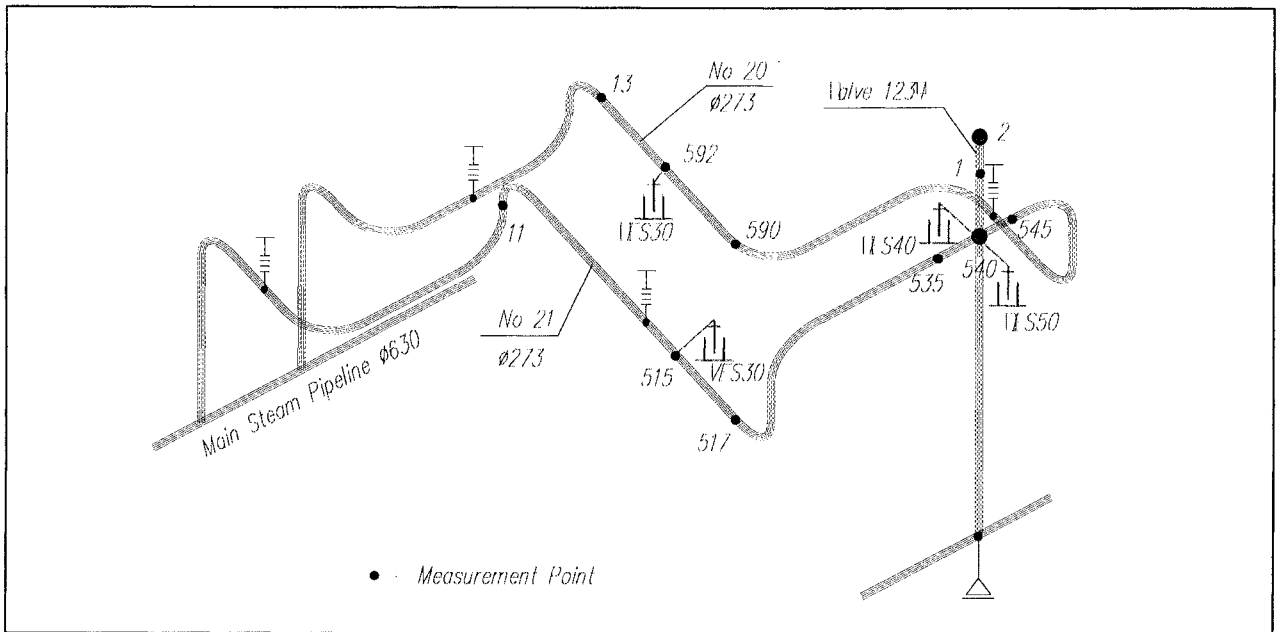
Figure 1. Measurement Points and Location of Dampers on Pipeline Section 12 Chernobyl NPP Unit 3.
