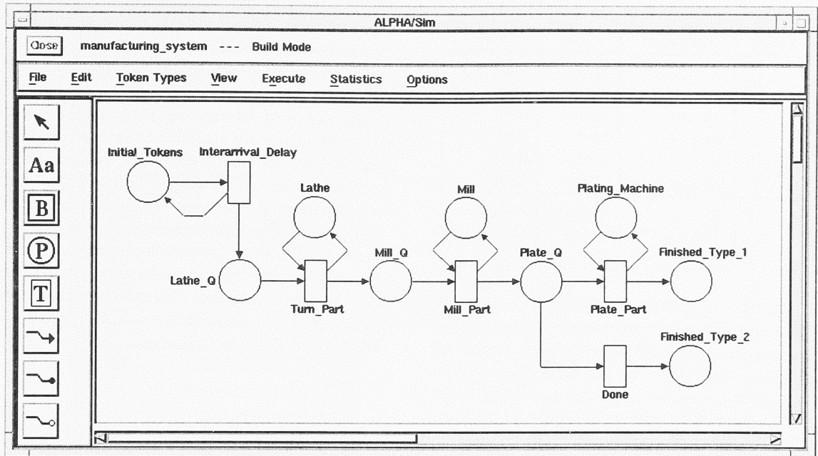
Figure 5: Completed Model
