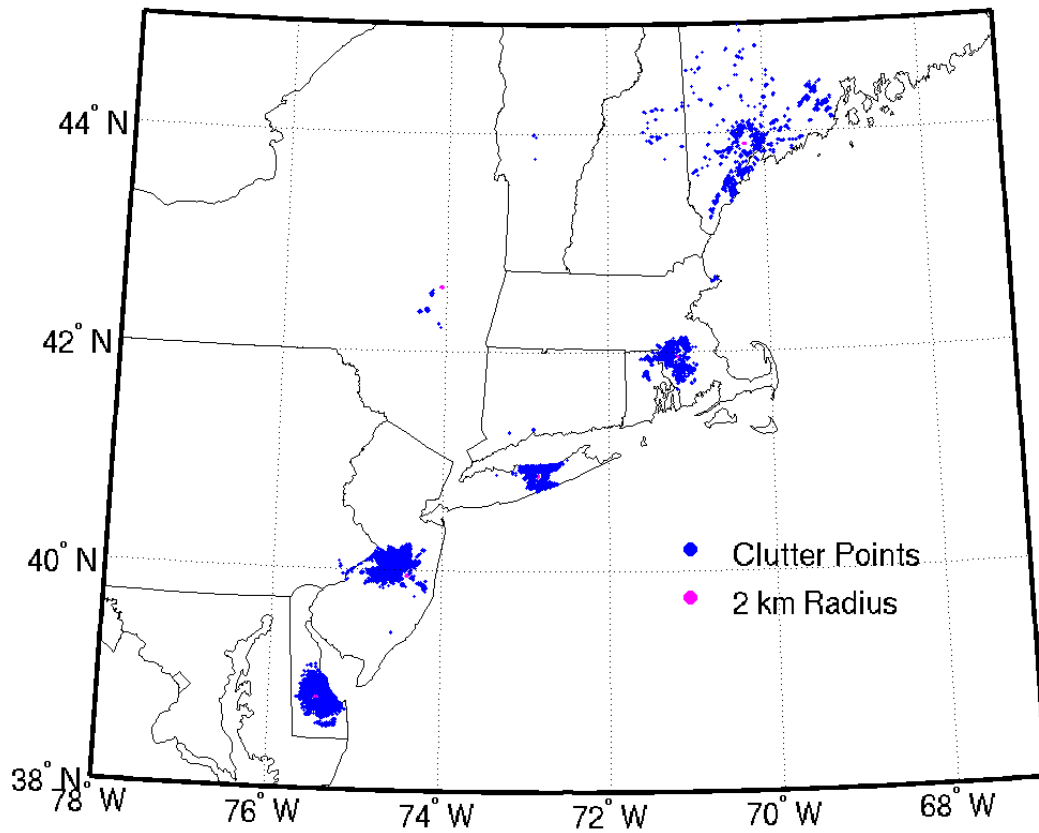
Figure 2.2 Pink dots represent the 2 km radius directly surrounding each radar. The blue dots denote clutter points removed due to persistent non-meteorological echo.
