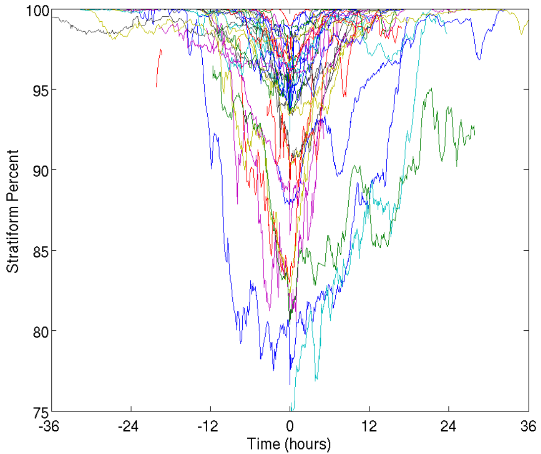
Figure 3.2 Time series of percent of total precipitation that is stratiform for storms containing only snow (34 storms). The time series are adjusted so that time=0 corresponds to time of the minimum percent of stratiform precipitation.
