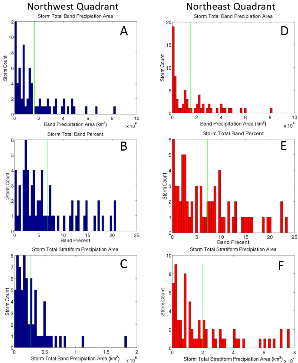
Figure 3.1 Distributions of band area (km 2 ), the percentage of the total precipitation area that is classified as bands, and stratiform area (km 2 ) summed over individual storm durations for the northwest and northeast quadrants. (A) Storm total band precipitation area for the northwest and the (D) northeast quadrants. (B) The band percentage of the storm total precipitation area for the northwest and the (E) northeast. (C) The storm total stratiform precipitation area for the northwest and (F) northeast Green lines represent the mean value for each plot.
