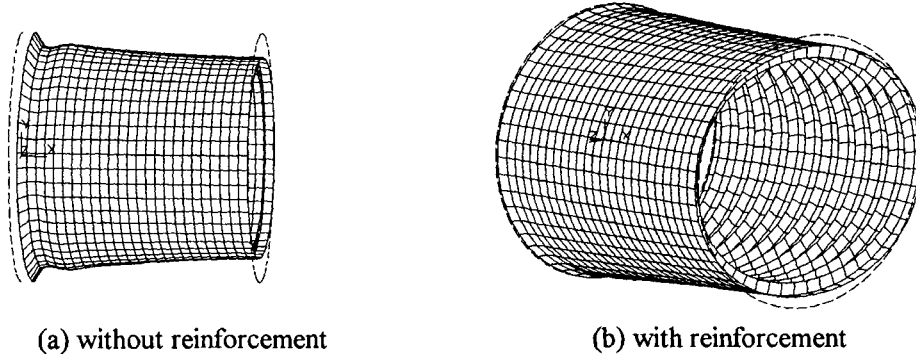
Figure 4: Displacements of the shell ( n = 2 waves)
