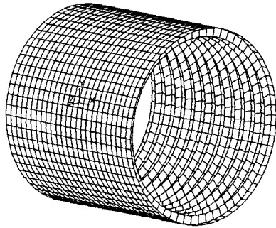
Figure 1: General dimensions and finite element model of the ring-stiffened cylindrical shell
