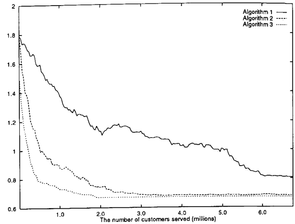
Figure 2: Performance of Algorithms 1, 2, and 3 using the neighborhood structure N_1 . The estimated objective function value at the global optimal solution is \hat{f}^* = 0.6717 .
