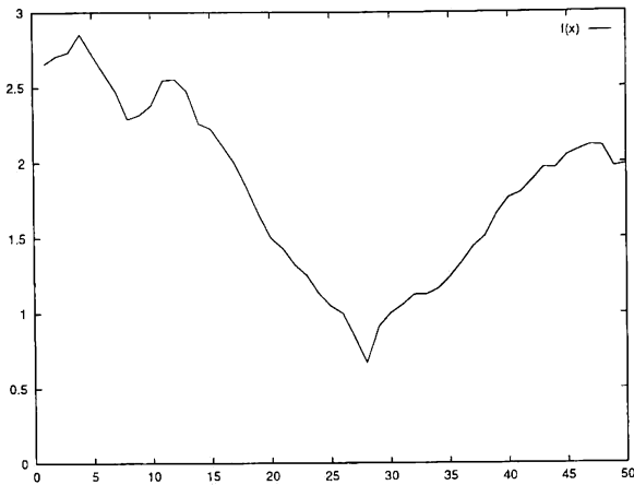
Figure 1: The estimated objective function values f(x) = E[W(x)] for all x \in S .
