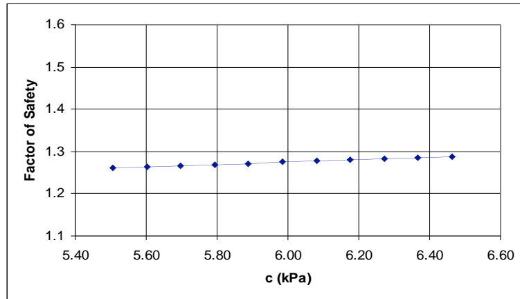
Figure 4. Effect of changing cohesion c of zone IIa saprolite soil on factor of safety
