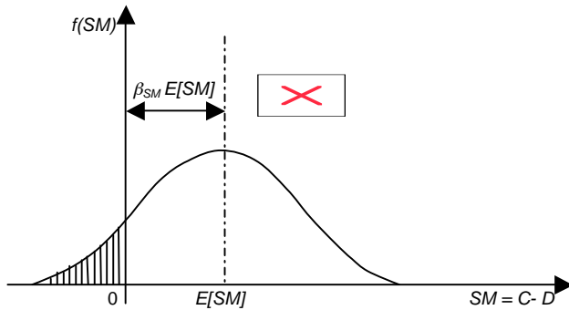
Figure 1. Reliability index of safety margin
