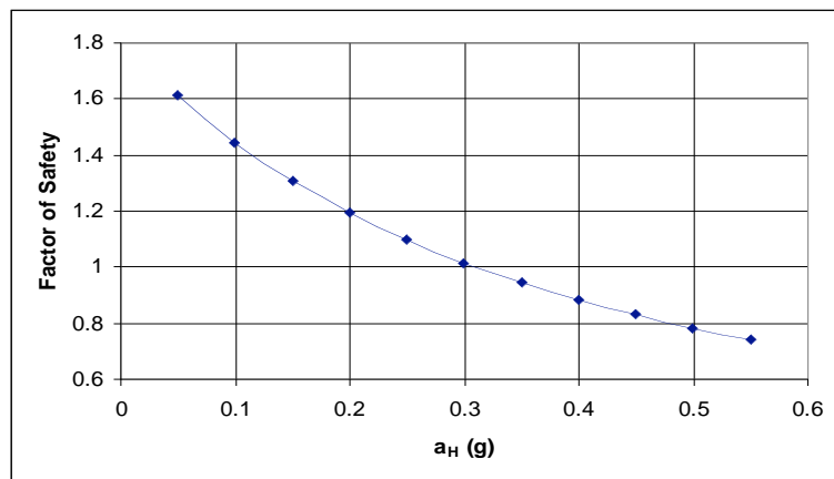
Figure 6. Effect of changing Horizontal Seismic Load on factor of safety
