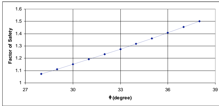
Figure 3. Effect of changing internal friction angle \phi of zone IIa saprolite soil on factor of safety
