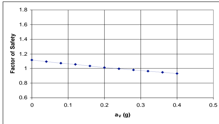
Figure 7. Effect of changing Vertical Seismic Load on factor of safety
