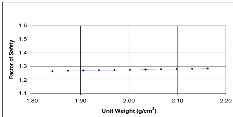
Figure 5. Effect of changing unit weight of zone IIa saprolite soil on factor of safety
