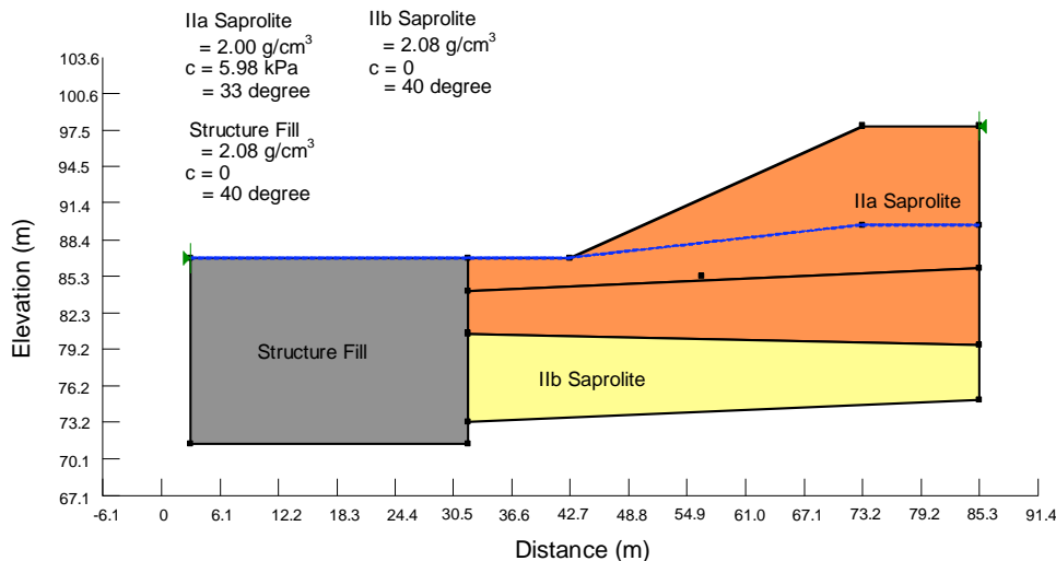
Figure 2. Cross section, material properties of a slope used in slope stability analysis
