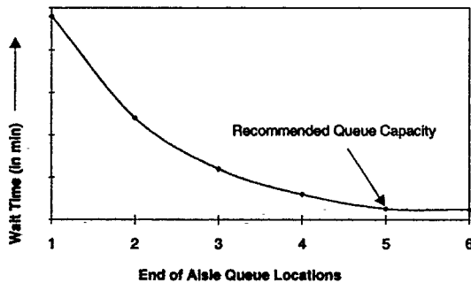
Figure 4: Vehicle Wait Time vs. End of Aisle Queues
