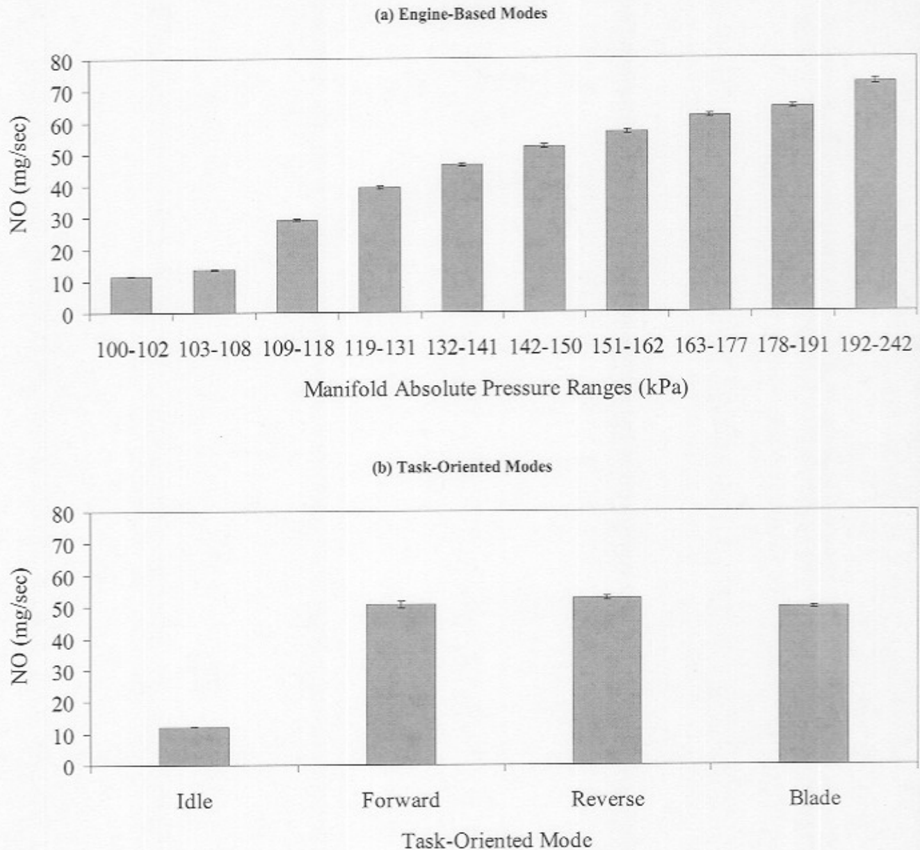
Figure 1. Average NO Emission Rates Measured on September 28, 2005 for a Bulldozer for (a) Engine-Based Modes and (b) Task-Oriented Modes
