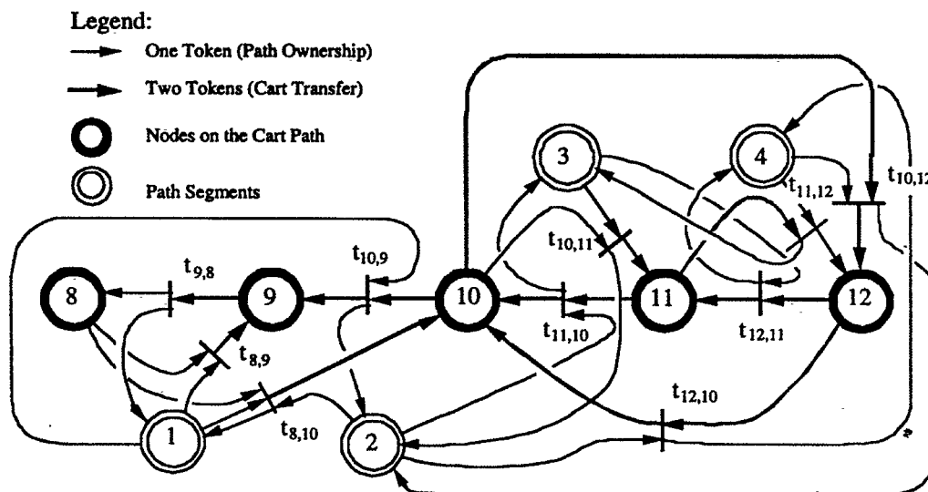
Figure 2: Petri-Network Control Logic for Allocating the Path Segments during AGV Transitions
