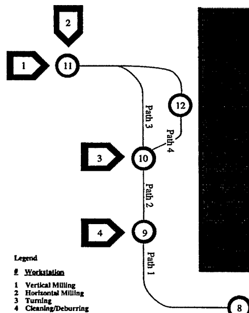
Figure 1: Schematic Layout for the AMRF
