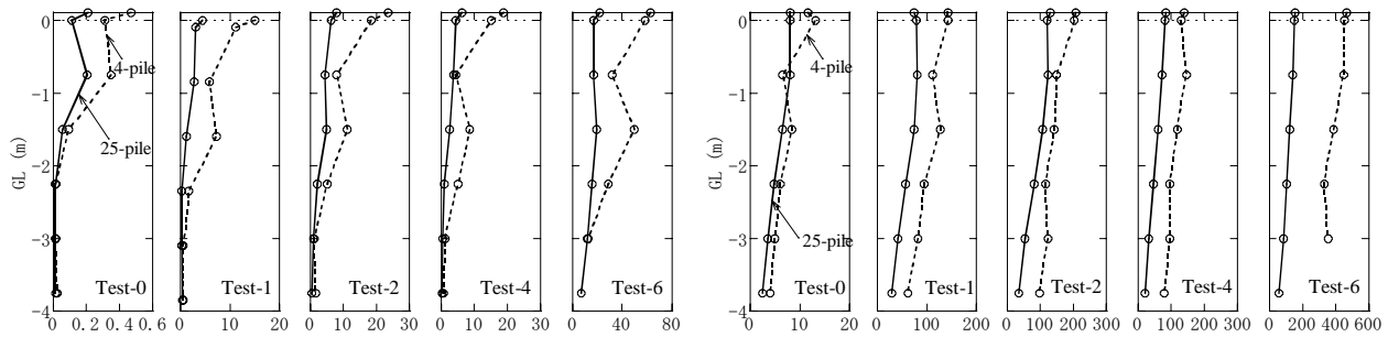
Max Bending Moment Max Axial Force Figure 21 Vertical Distributions of Bending Moments and Axial Forces (25-Pile Structure : Pile A4, 4-Pile Structure : Pile A1 )
