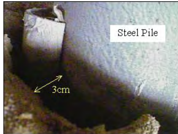
Figure 10 Spaces generated during Test-2
