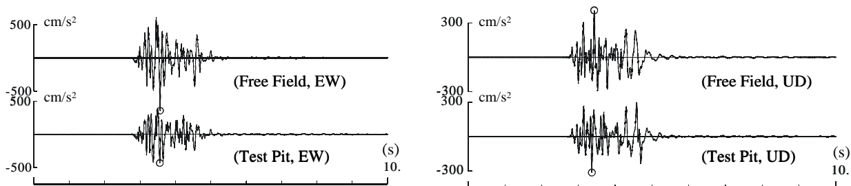
Figure 14 Acceleration Records at Surface of Test Pit and Adjacent Free Field (Test-2)
