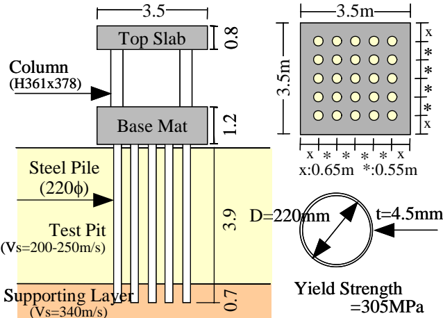
Figure 3 Details of 25-pile Structure
