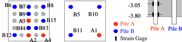
Figure 5 Locations of Strain gauges
