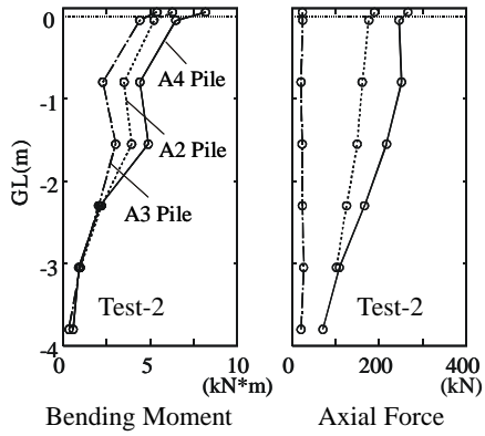
Figure 24 Vertical Distribution of Maximum Bending Moment and Axial force
