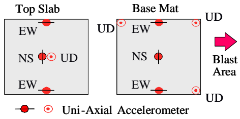
Figure 4 Locations of Accelerometers
