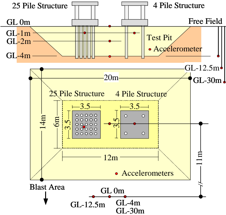
Figure 2 Test Pit and Test Structures
