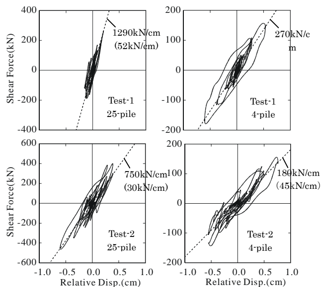
Figure 20 Relationship between inertia forces ( Q ) of test structure and relative displacements ( d ) between base mat and test pit surface.
