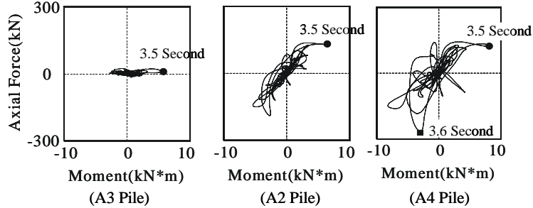
Figure 26 Moment-Axial force Relationship at Different Locations for Test-2
