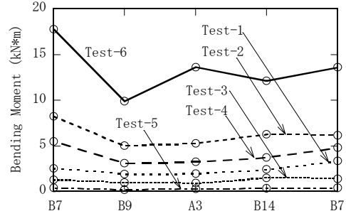
Figure 25 Distribution of Maximum Bending Moment along Line-1
