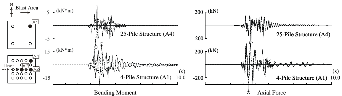
(Solid Line: Records at GL+0.05m / Dotted Line: Records at GL-1.55m) Figure 22 Time Histories of Bending Moment and Axial Force for Test-2
