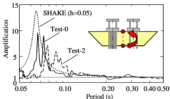
Figure 16 Amplifications obtained from Fourier Spectra
