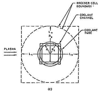
2. Schematics of cylindrical and rectangular breeder cell models.
