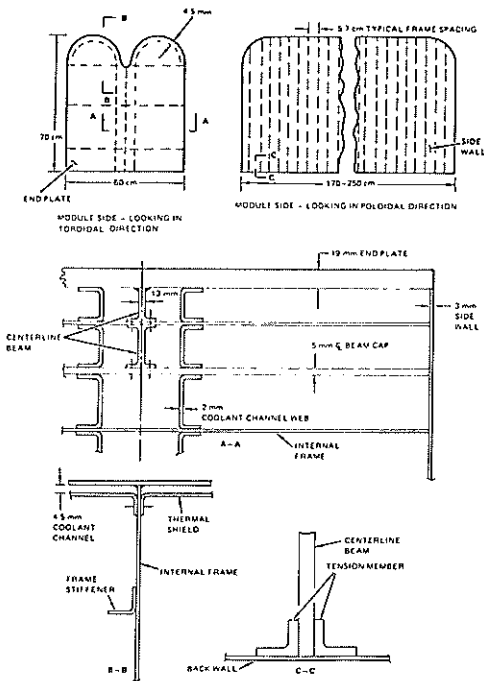
7. Structural sizing for Li-Pb self-cooled blanket concept.
