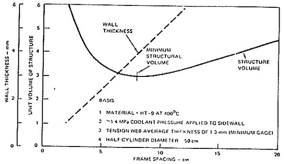
8. Frame spacing in Li-Pb self-cooled blanket for minimum structural volume.
