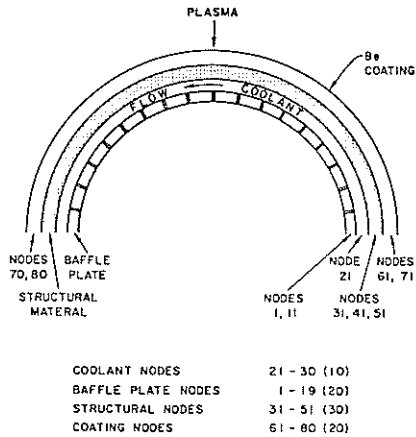
6. Liquid breeder blanket thermal-hydraulic model showing distribution of node points.
