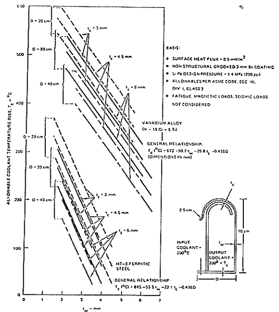
9. Allowable relationships of blanket parameters.
