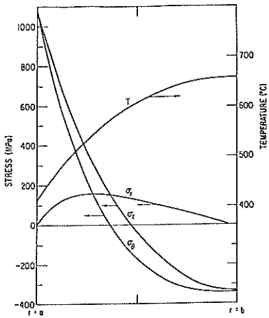
3. Calculated radial temperature and thermoelastic stress distribution in Region 1 of the blanket (thick, hollow-cylinder model).
