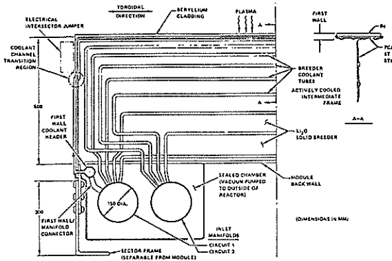
1. DEMO Li_2O solid breeder blanket concept.
