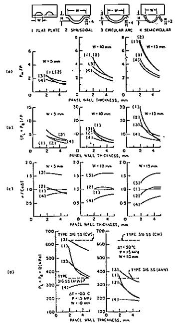
4. (a) Maximum primary membrane stress intensities. (b) Maximum primary membrane local plus bending stress intensities. (c) Thermal stresses. (d) Maximum primary local membrane plus bending plus secondary stress and 3 S_0 allowable stresses.
