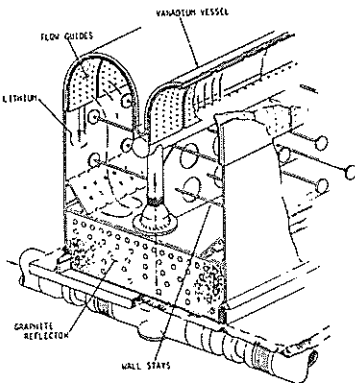
5. DEMO liquid breeder blanket concept.
