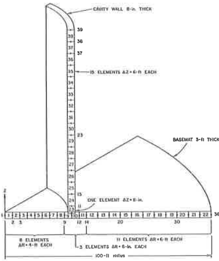
Fig. 2. Structural Finite Element Mesh
