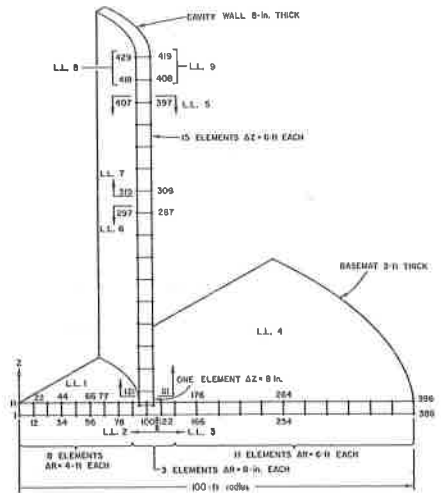
Fig. 3. Thermal Finite Element Mesh (10 thermal elements per structural element)
