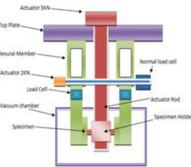
Figure-3: Schematic of experimental set-up
