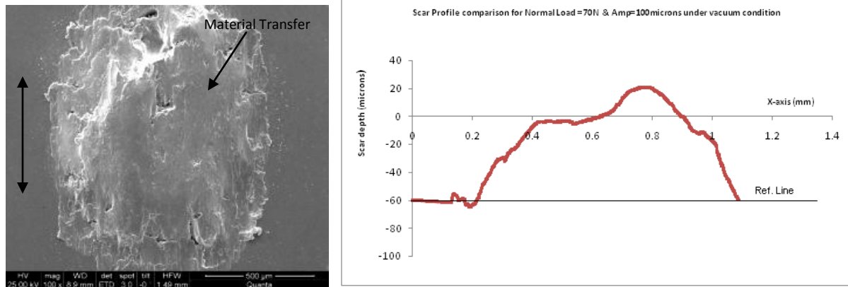
(a) (b) Figure-8: (a) SEM micrographs (b) Scar profile of self mated SS316L for normal load of 70N under vacuum condition for displacement amplitude of 100microns (Note- Arrow indicates fretting direction)
