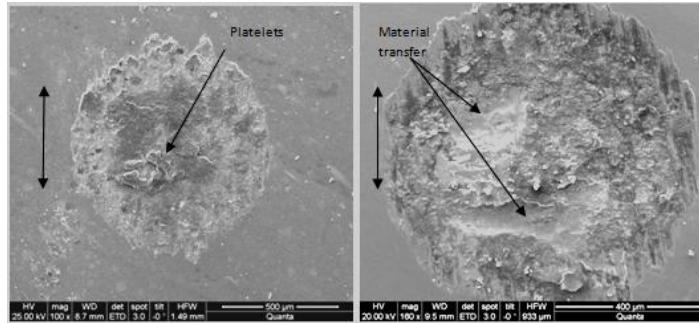
Figure-6: SEM micrographs of self mated SS316L for normal load of 70N and displacement amplitude of 50 microns under ambient condition for (a) Flat (b) Pin surfaces. (Note- Arrow indicates fretting direction)
