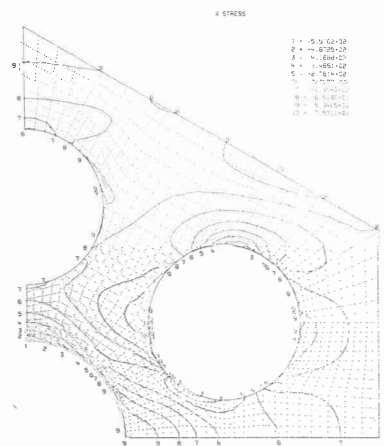
Fig. 6 Contour Plot of \sigma_{XX} Eight Divisions of Eight-Node Quads
