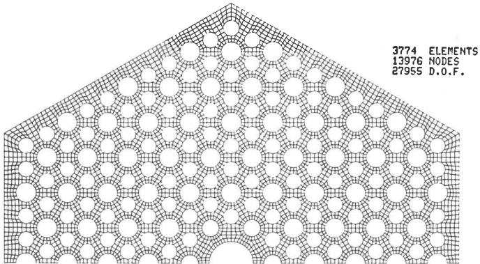
Fig. 2 Mesh for Standard Fuel Element
