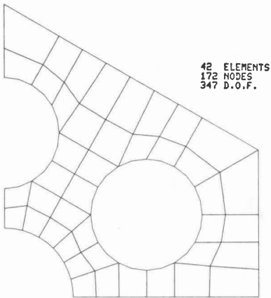
Fig. 3 One Quarter of a Seven-Hole Block Two Divisions of Eight-Node Quads Across Minimum Web
