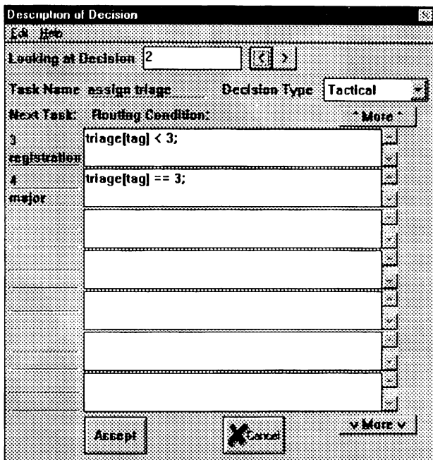
Figure 4: Micro Saint Tactical Decision
