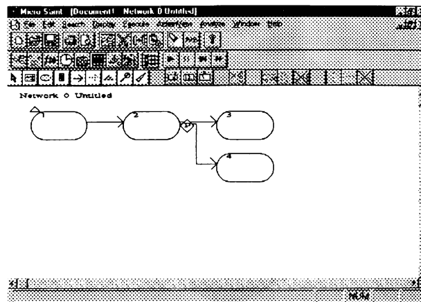
Figure 3: Micro Saint Tool Palette
