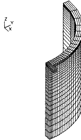
Figure 2: Finite element model of the lug-cylinder attachment
