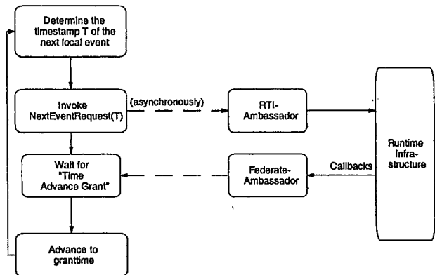
Figure 2: Principle of the Synchronization Thread
