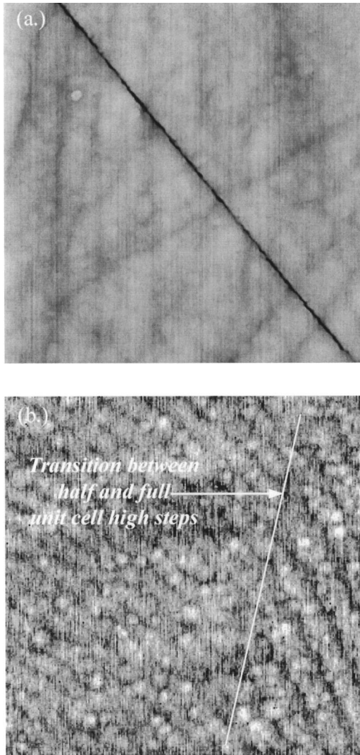
FIG. 6. (a) 10\ \mu\text{m} \times 10\ \mu\text{m} AFM scan of MOVPE grown AlN on an unetched 6H-SiC(0001). The rms roughness value is 1 nm; (b) 10\ \mu\text{m} \times 10\ \mu\text{m} AFM scan of MOVPE grown AlN on an etched 6H-SiC(0001) with (N_D - N_A) = 8.7 \times 10^{17}\ \text{cm}^{-3} . The arrow indicates the transition region between unit cell high and one-half unit cell high steps on the surface. The rms roughness value is 0.4 nm.
