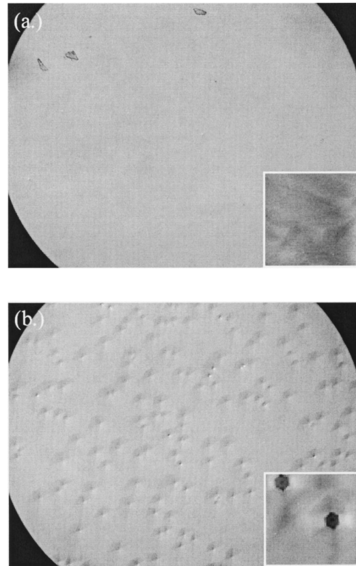
FIG. 7. (a) 200\times optical microscope images of MOVPE grown AlN on a hydrogen etched 6H-SiC(0001) substrate with (N_D - N_A) of (a) 8.7 \times 10^{17}\ \text{cm}^{-3} ; (b) 2.8 \times 10^{18}\ \text{cm}^{-3} . The inset in each figure shows a 35\ \mu\text{m} \times 35\ \mu\text{m} AFM image of the respective surface.
