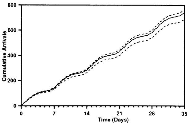
Figure 9: 90% Tolerance Interval for \mu(t) , t \in (0, 35]
