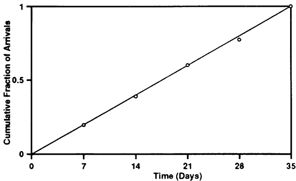
Figure 2: Fitted Function at Resolution 0, \hat{R}_0(s)
