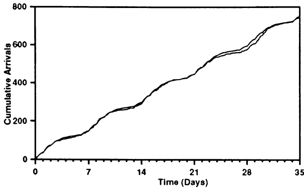
Figure 8: Fitted Mean-Value Function, \hat{\mu}(t) (Smooth Curve) Superimposed on Observed Cumulative Number of Arrivals (Step Function)
