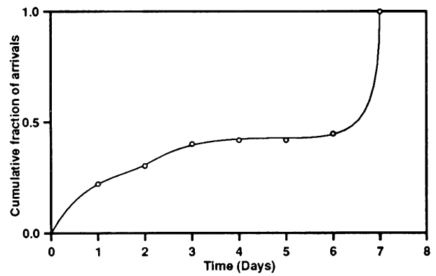
Figure 13: Resolution 1 Function \hat{R}_1(\cdot) Fitted to the Cumulative Fraction of Arrivals at the End of Each Day of the Week
