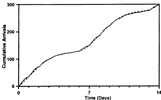
Figure 7: Fitted Mean-Value Function at Resolution 2, \hat{\mu}_2(t) (Solid Line) Superimposed on \hat{\mu}_1(t) (Dashed Line)
