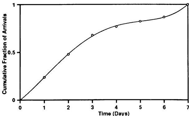
Figure 3: Fitted Function at Resolution 1, \hat{R}_1(s)
