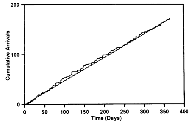
Figure 15: Fitted Mean-Value Function Using Heuristic Method
