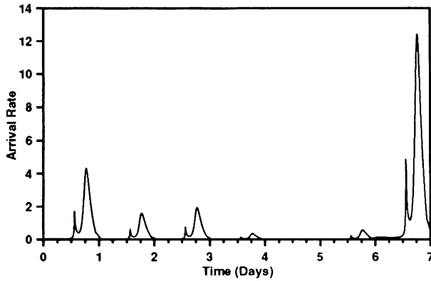
Figure 17: Fitted Weekly Rate Function Using Heuristic Method
