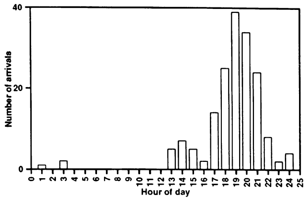
Figure 10: Histogram of the Number of Arrivals to Transplant Center 11 by Hour of the Day during 1992
