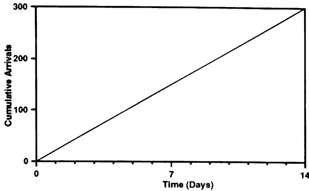
Figure 5: Fitted Mean-Value Function at Resolution 0, \hat{\mu}_0(t)
