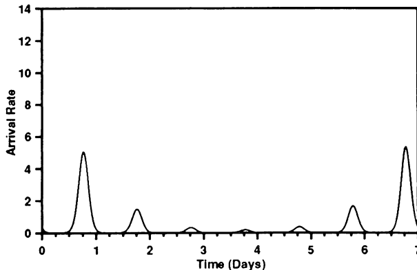
Figure 18: Fitted Weekly EPTMP Rate Function
