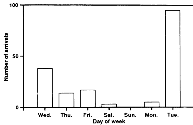
Figure 11: Histogram of the Number of Arrivals to Transplant Center 11 by Day of the Week during 1992
