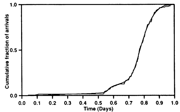
Figure 14: Resolution 2 Curve versus the Cumulative Fraction of Arrivals over the Period of One Day
