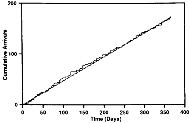
Figure 16: Fitted EPTMP Mean-Value Function
