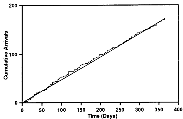
Figure 12: Fitted Mean-Value Function \hat{\mu}(\cdot) at Resolution 0 versus the Cumulative Number of Arrivals over the Interval (0, 366]
