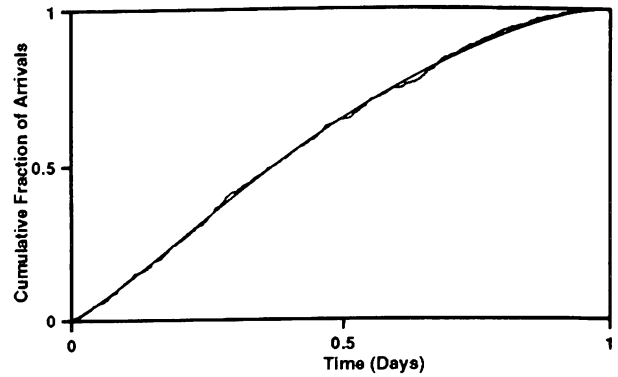
Figure 4: Fitted Function at Resolution 2, \hat{R}_2(s)
