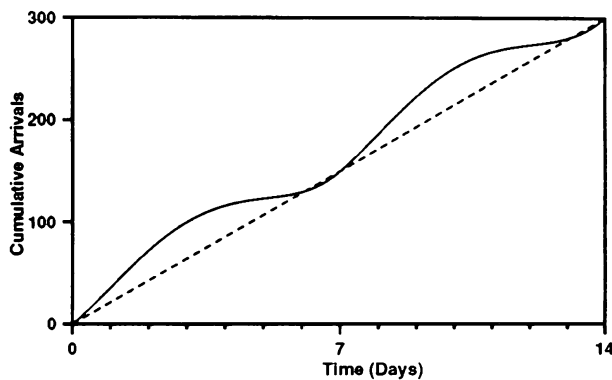
Figure 6: Fitted Mean-Value Function at Resolution 1, \hat{\mu}_1(t) (Solid Line) Superimposed on \hat{\mu}_0(t) (Dashed Line)
