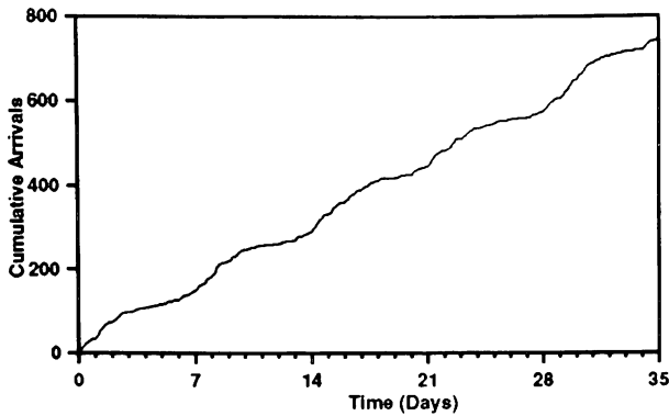
Figure 1: A Realization of the NHPP Having a Linear Trend and Two Periodicities
