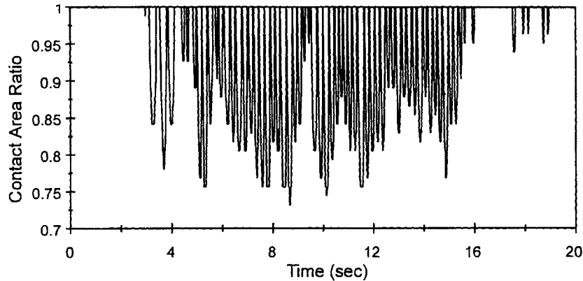
Figure 5: Percentage of bottom plate area in contact with the foundation
