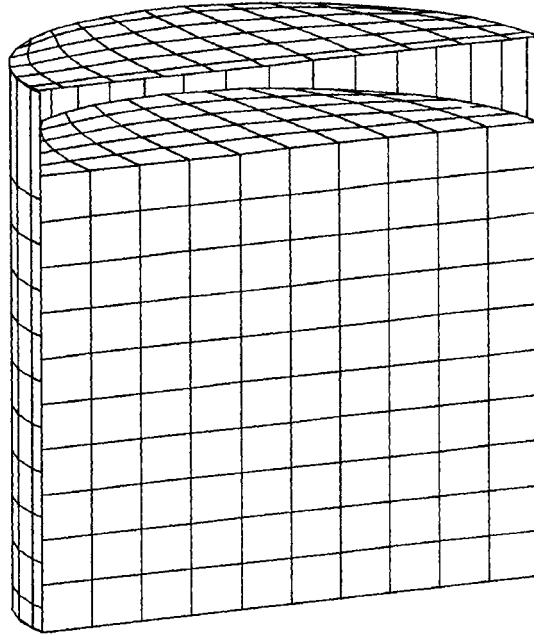
Figure 1: Finite element mesh of the coupled liquid-tank system
