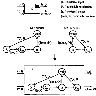
Figure 2: DEVS Simulator Algorithm
