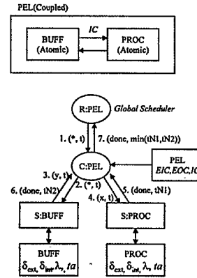
Figure 3: Hierarchical Simulation Algorithm for DEVS Coordinator
