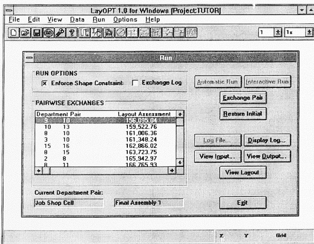
Figure 2: Interactive Run
