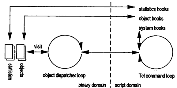
Figure 5: The Operation of GMSim
