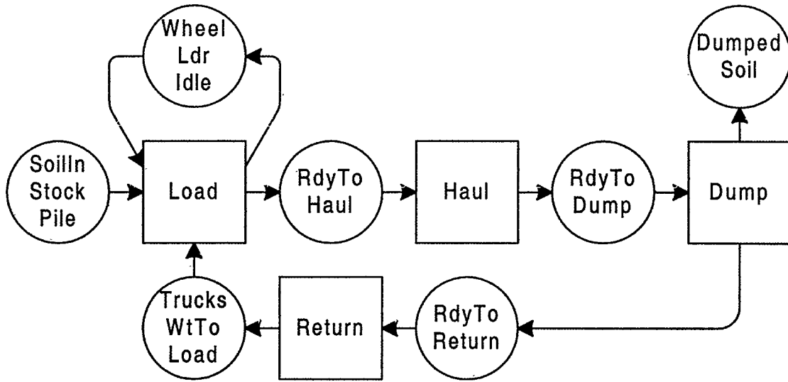
Figure 1 - Conventional ACD for earthmoving operation
