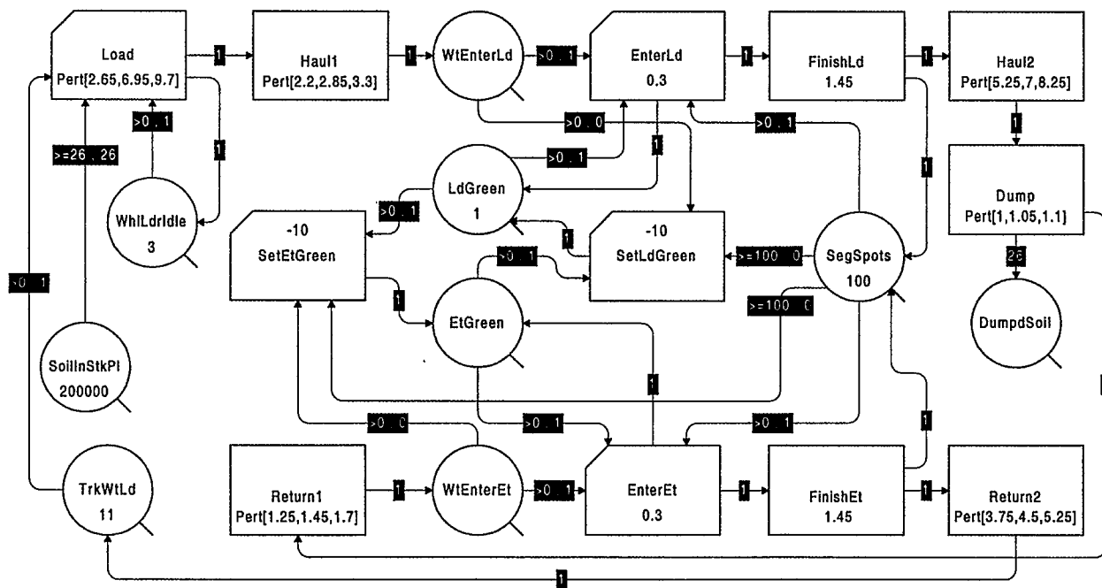
Figure 5 - ACD for Earthmoving Operation With Unidirectional Narrow Segment
