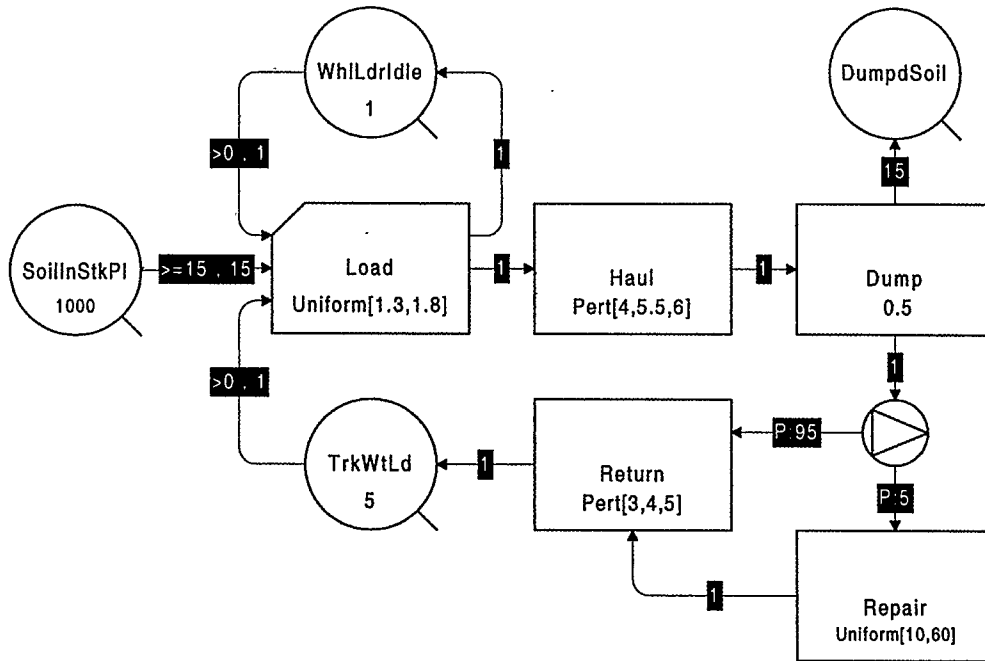
Figure 4 - ACD for Earthmoving Operation With Truck Breakdown and Repair
