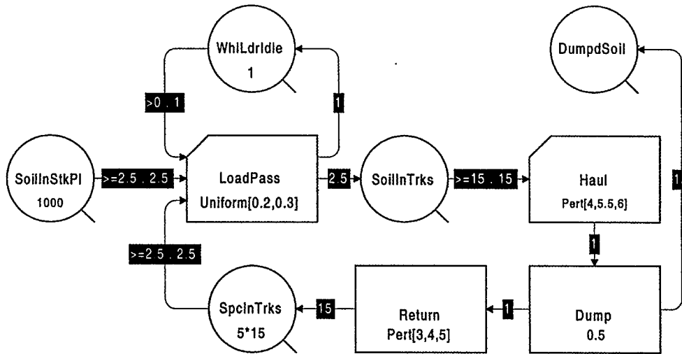
Figure 3 - ACD for Earthwork Operation With Multiple Loader Passes
