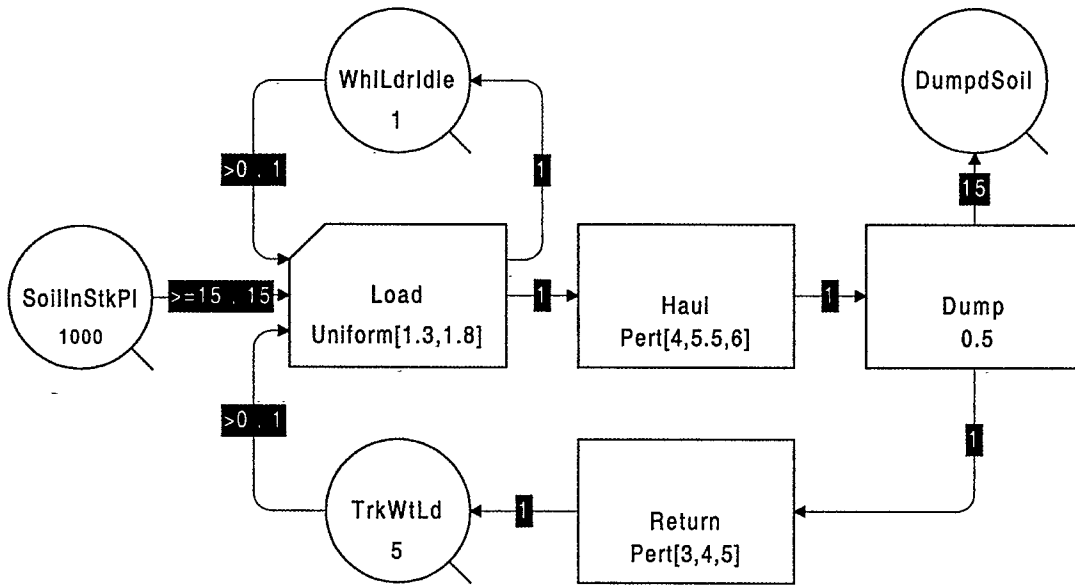
Figure 2 - EZStrobe ACD for earthmoving operation
