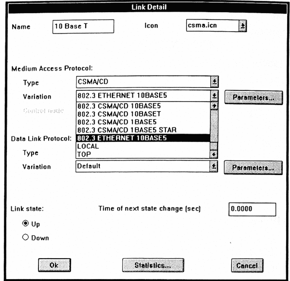
Figure 3: Editing a CSMA/CD link
