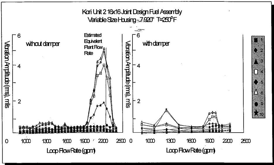
Fig. 6. Variable Pitch FACTS Loop Test Result.
