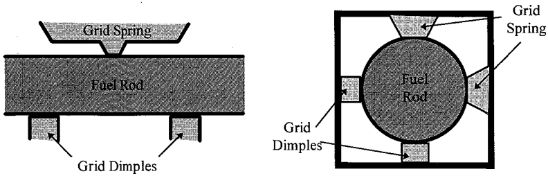
Fig. 1. Fuel Rod Contact Geometry
