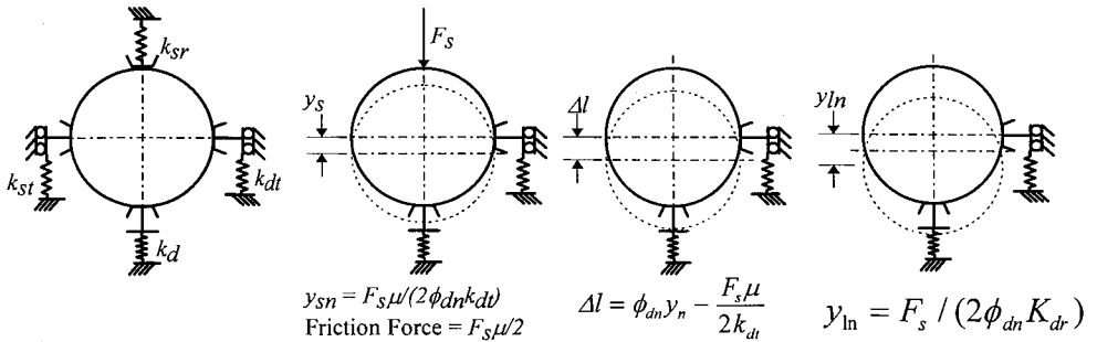
Fig. 1. Fuel Rod Contact Geometry
