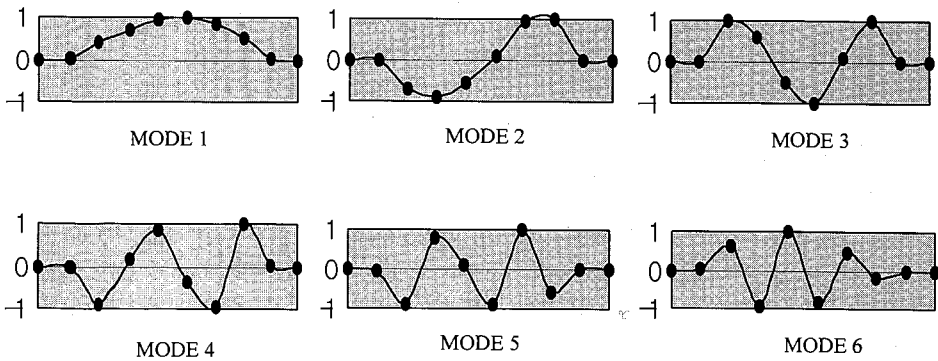
Fig. 5. Vibration Mode & Amplitude.
