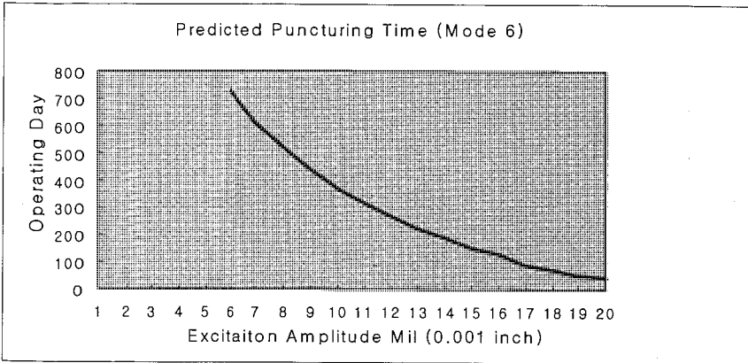
Fig. 3. Predicted Puncturing Time
