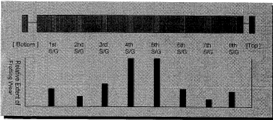
Fig. 2. Relative Fretting Wear Volume from PIE result
