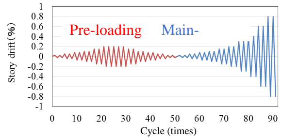
Figure 3 Loading history
