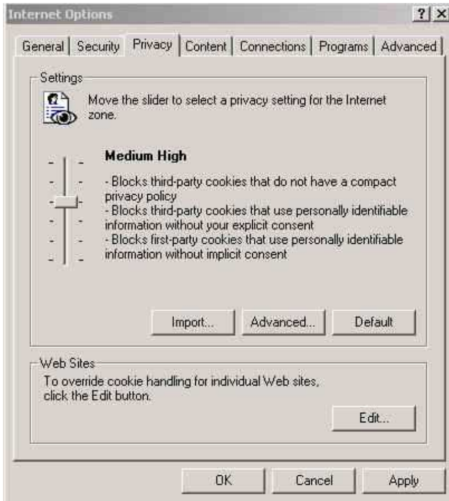
Figure 6.3 IE 6.0 Privacy Settings
