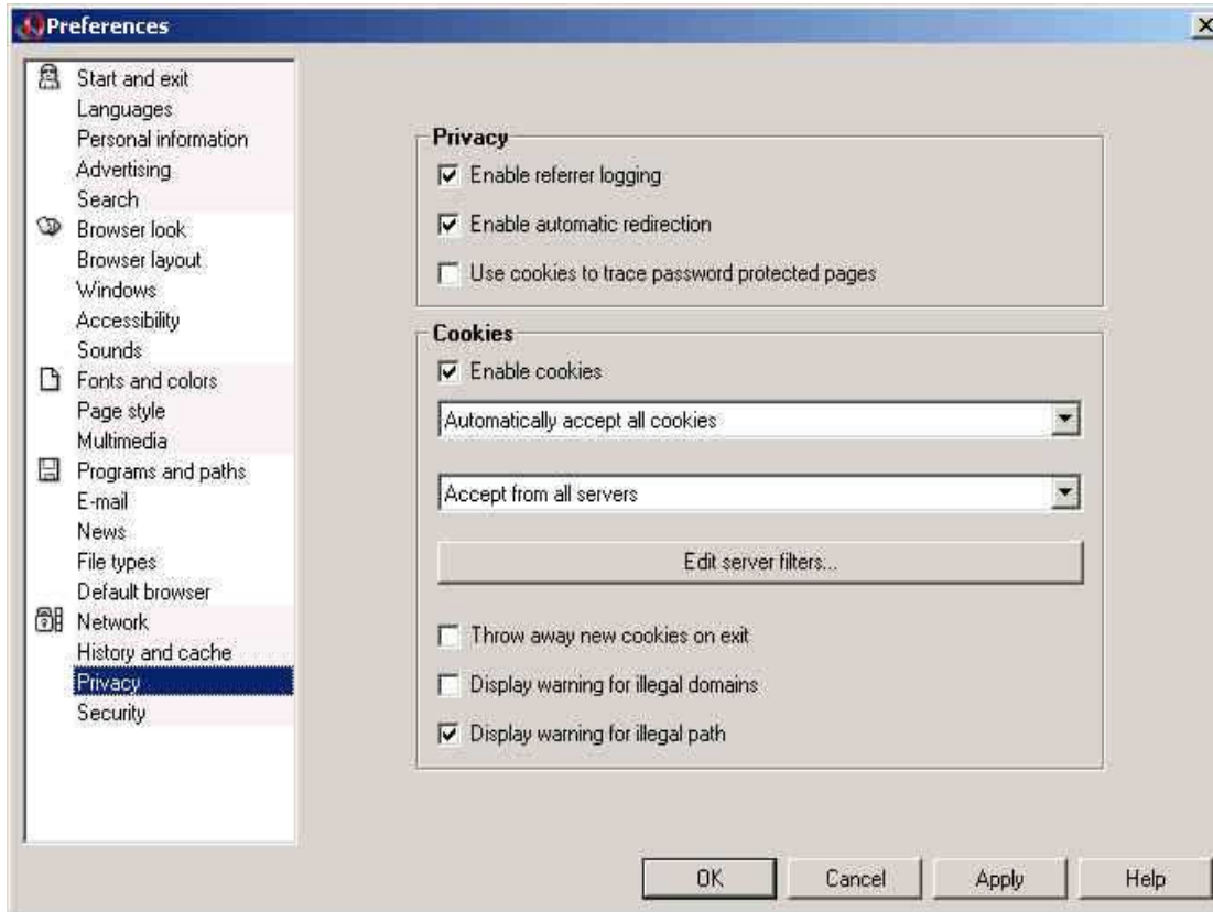
Figure 6.11 Opera 6.0 Privacy Settings
