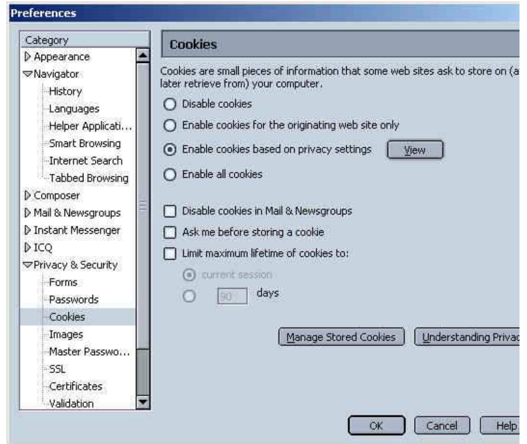
Figure 6.6 Netscape 7.0 PR1 Cookie Settings
