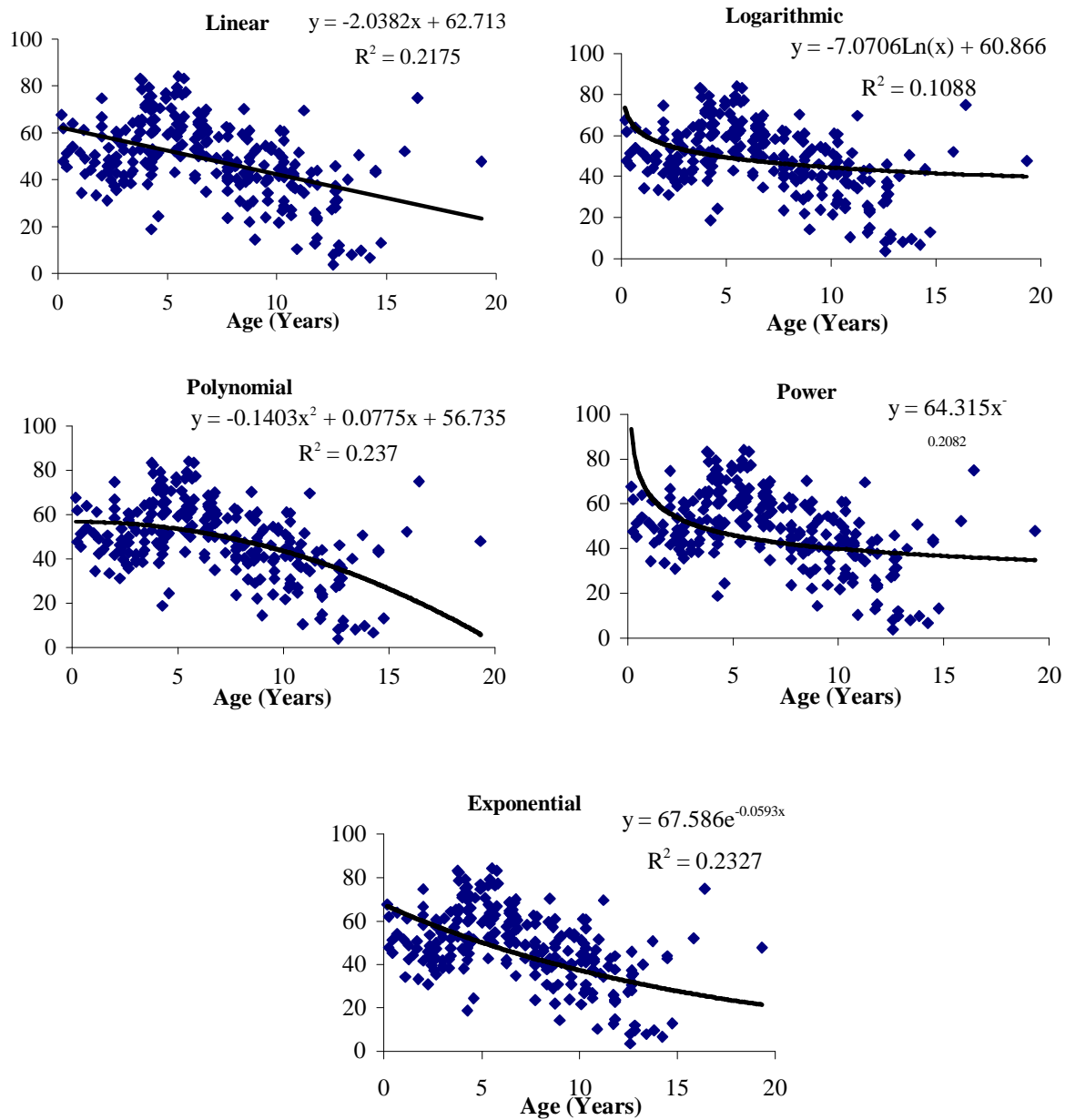
Figure 7.2. Deterioration Curves for Type I Yellow Sheeting
