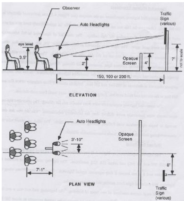
Figure 2.7. Laboratory Experimental Setup
