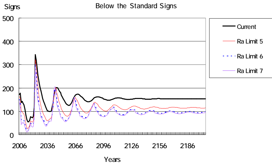
Figure 9.25. Changing Visual Inspection Rejection Threshold - Red Signs
