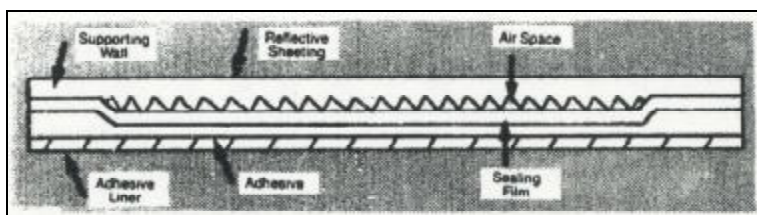
Figure 2.6. Prismatic Cube-Corner Sheeting [McGee, et. al. 1998a]
