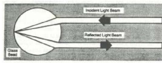
Figure 2.2. Glass Bead Retroreflection [Austin, et. al. 2001]
