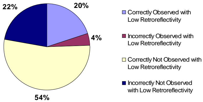
Figure 7.17. Type I Red Sheeting
