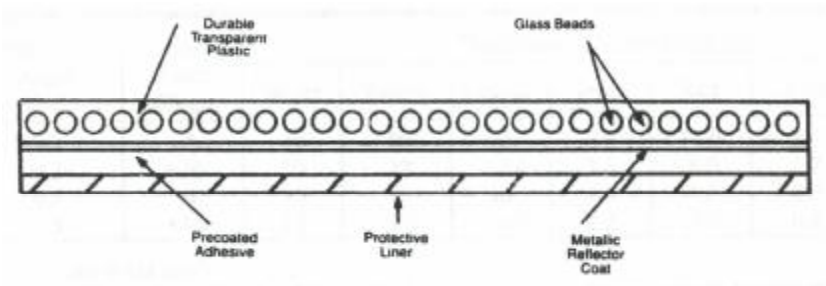
Figure 2.4. Enclosed Lens Sheeting [McGee, et. al. 1998a]
