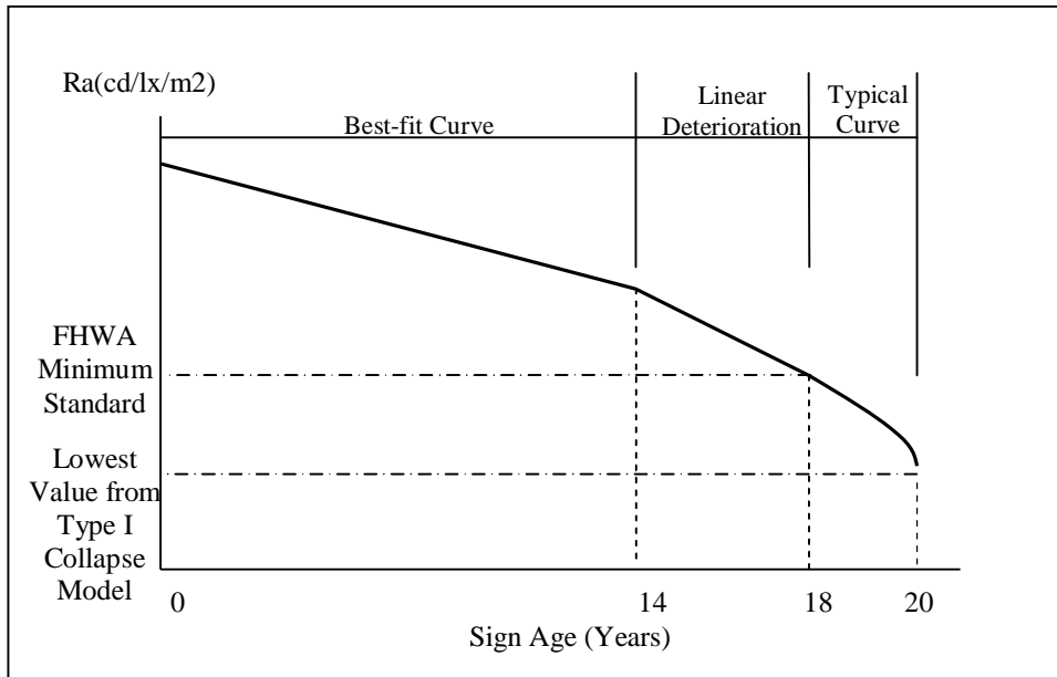
Figure 9.12. Typical Deterioration Curve for Type III Signs
