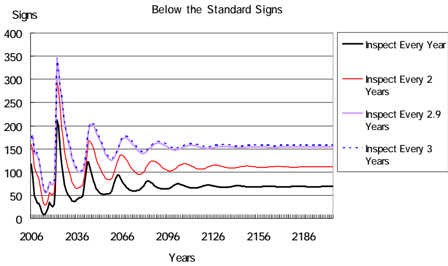
Figure 9.21. Inspection Frequency Adjustment - Red Signs
