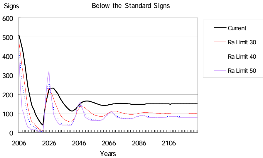
Figure 9.28. Changing Inspection Rejection Threshold while Using a Retroreflector - Yellow Signs
