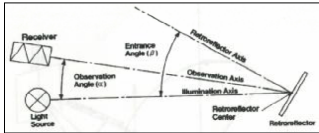
Figure 2.1. Basic Principles of Retroreflectivity
