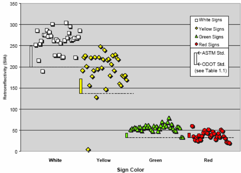
Figure 2.28. Retroreflectivity Values for Signs of Different Color
