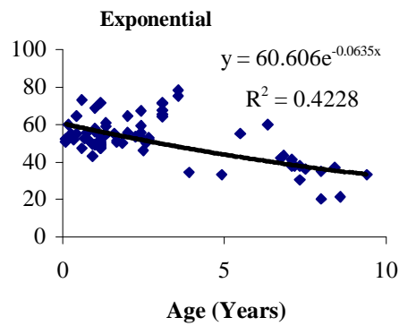
Figure 7.7. Deterioration Curves for Type III Red Signs
