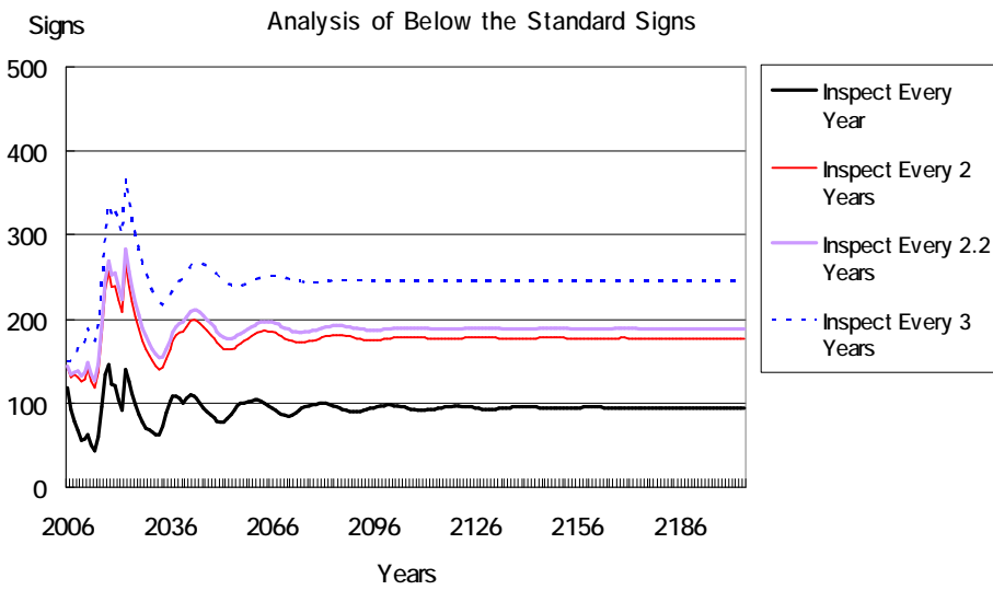
Figure 9.16. Simulation Results for Green Signs
