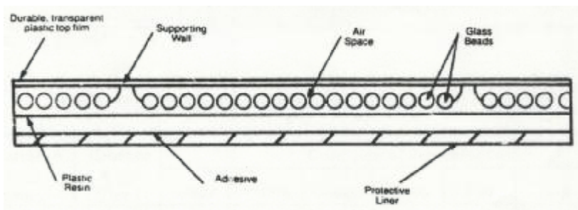
Figure 2.5. Encapsulated Lens Sheeting [Mc Gee, et. al. 1998a]
