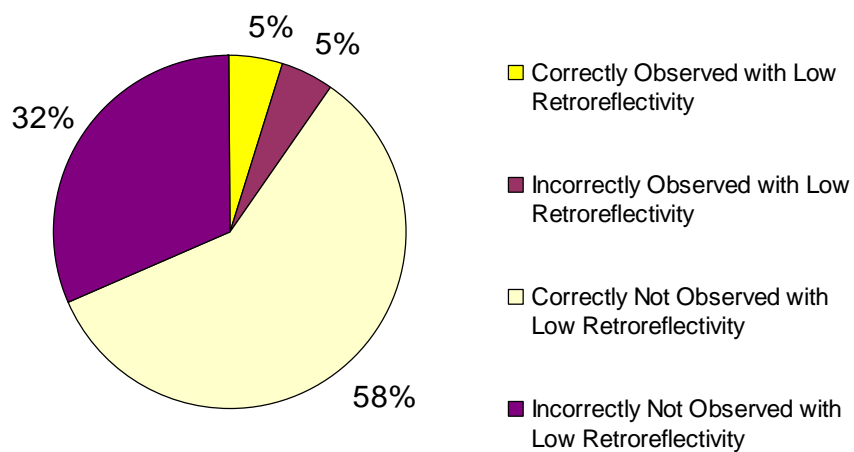
Figure 7.18. Type I Green Sheeting
