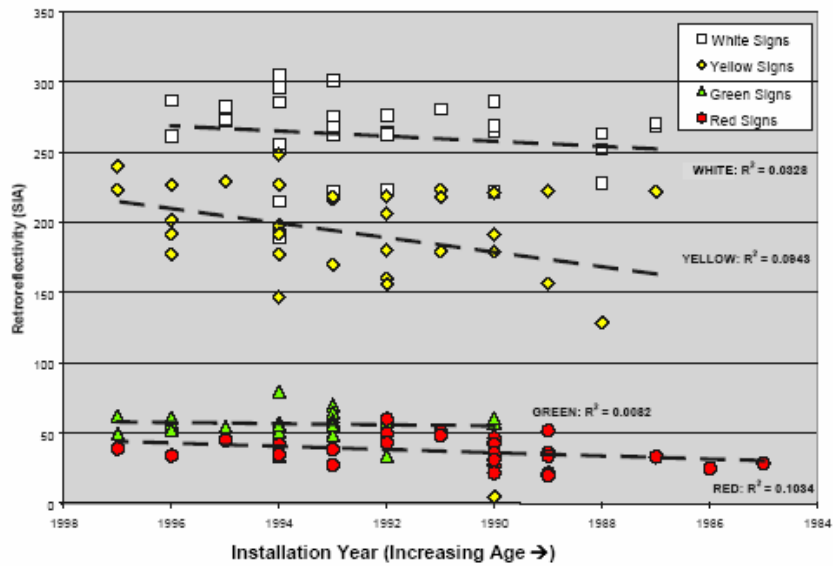
Figure 2.29. Retroreflectivity and Sign Age
