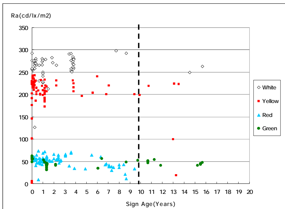
Figure 9.11. Type III Sign Field Data
