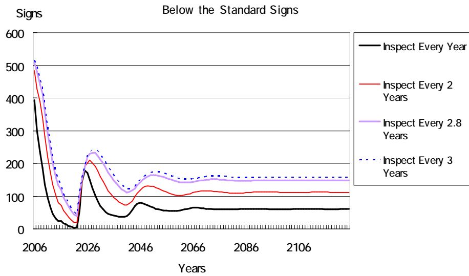
Figure 9.14. Simulation Results for Yellow Signs
