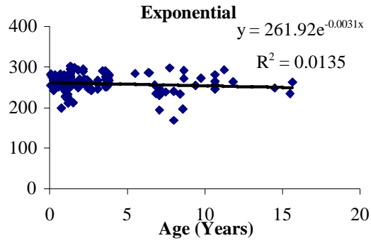
Figure 7.5. Deterioration Curves for Type III White Signs
