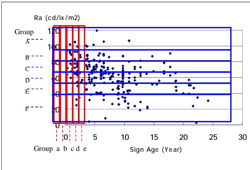
Figure 9.7. Group of Type I White Signs
