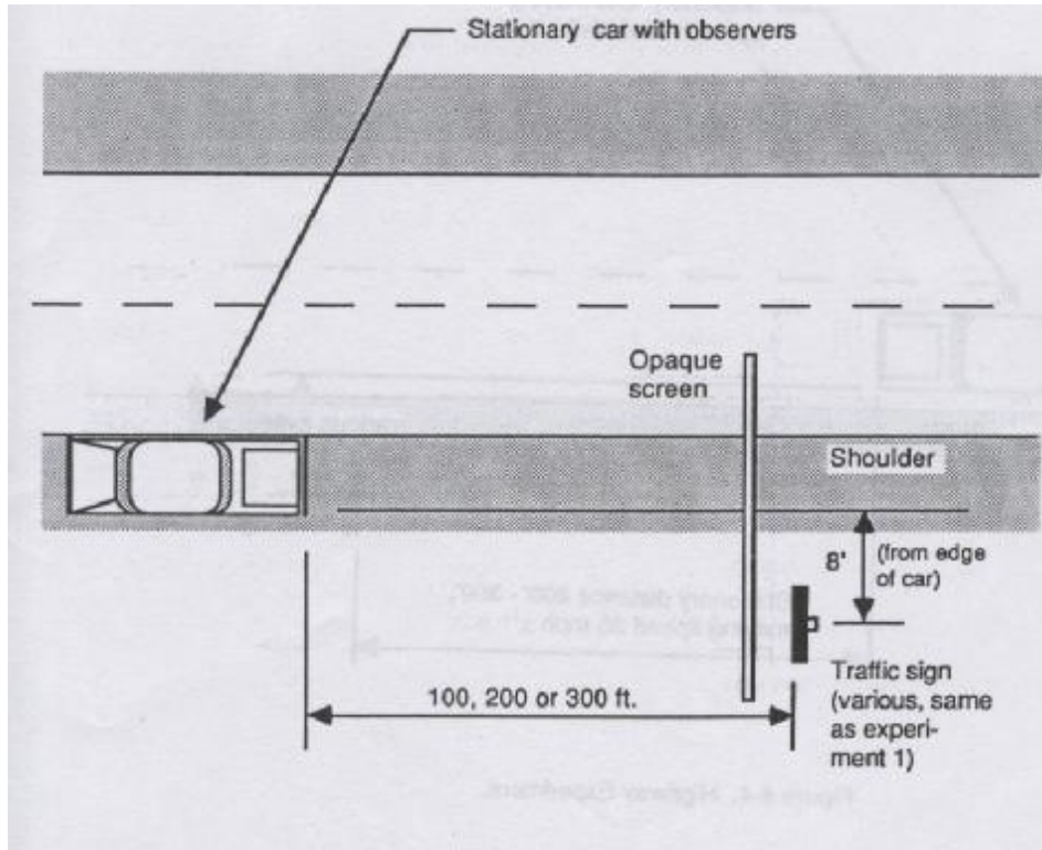
Figure 2.8. Controlled Highway Experiment
