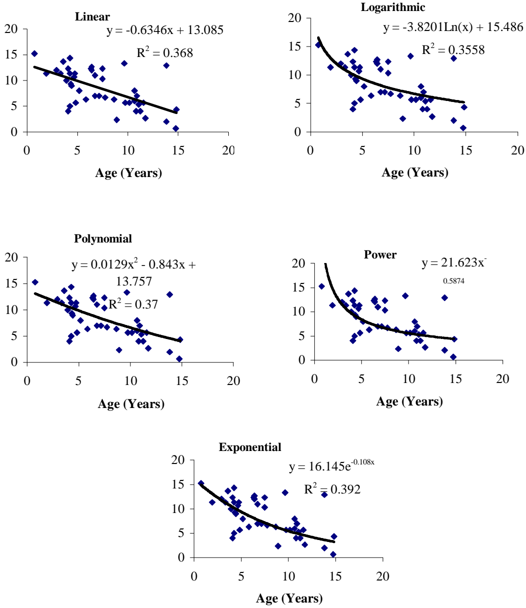
Figure 7.3. Deterioration Curves for Type I Red Signs
