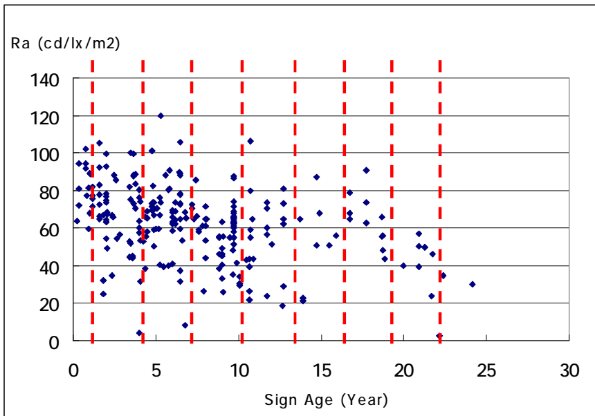
Figure 9.8. Separation of Type I White Signs
