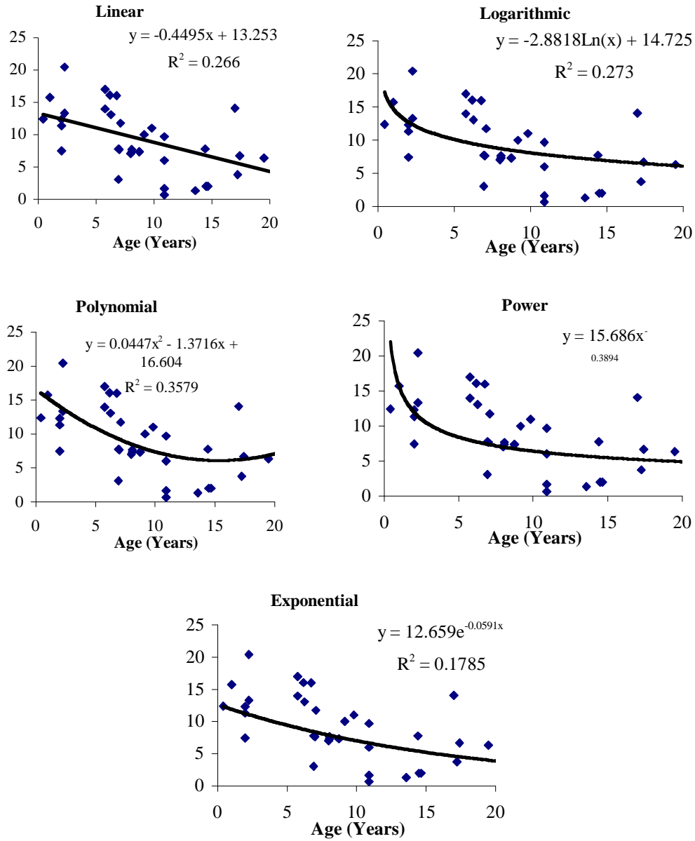
Figure 7.4. Deterioration Curves for Type I Green Signs
