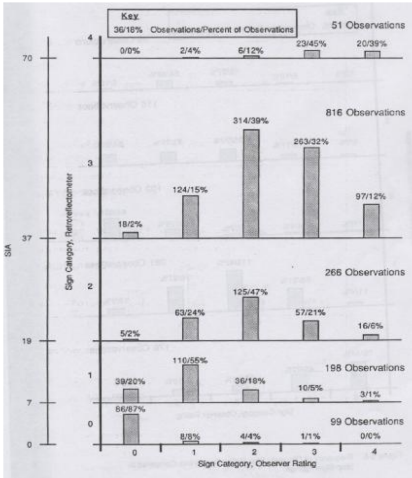
Figure 2.14. Frequency Distribution based on Sign Retroreflectivity
