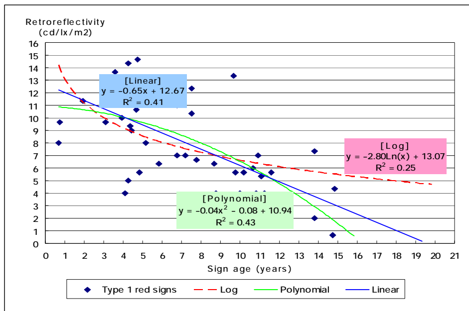
Figure 9.10. Various Deterioration Curves for Type I Red Sign from the NCSU Field Data
