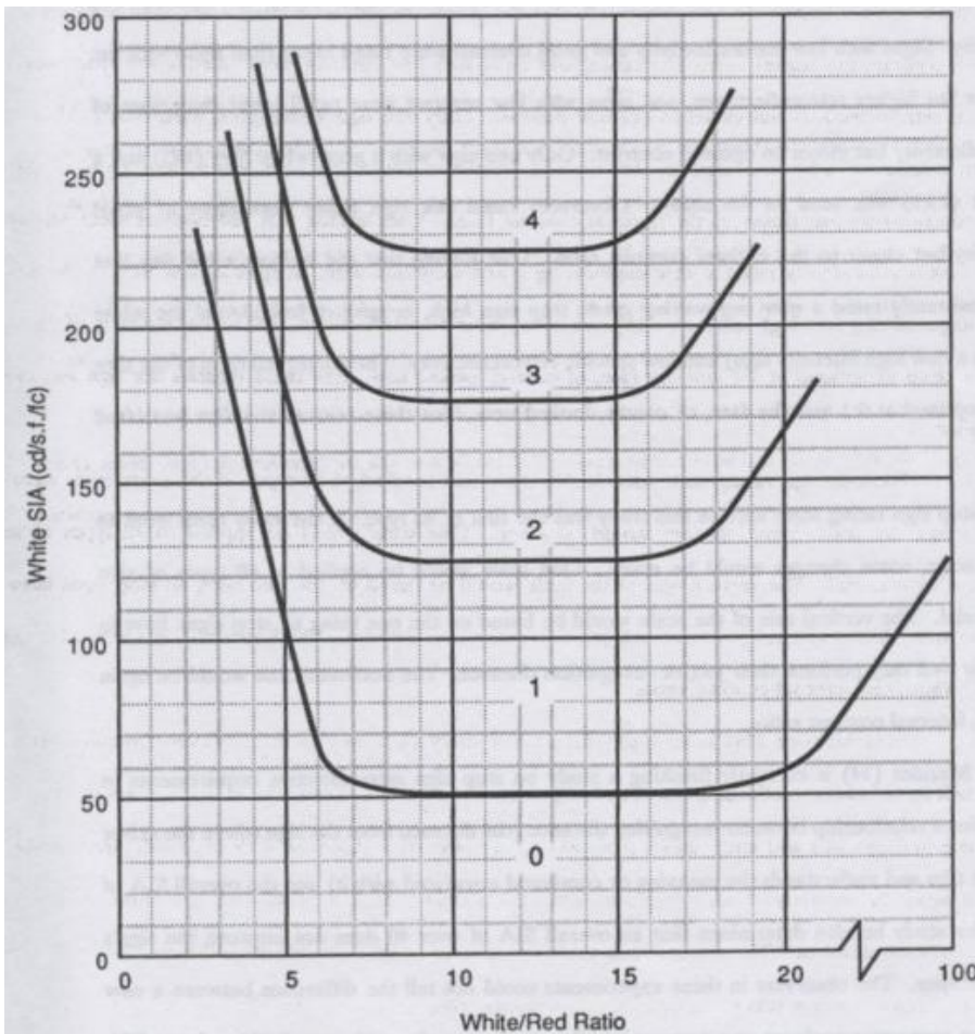
Figure 2.16. Stop Sign Rating Scale - All Sheeting Materials
