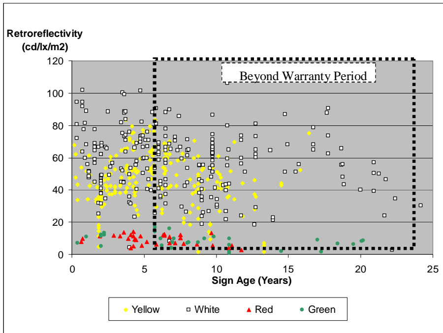
Figure 9.4. Type I Sign Data Distribution
