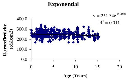
Figure 14.5. Curve Fitting for Type III White Signs (Purdue Study)
