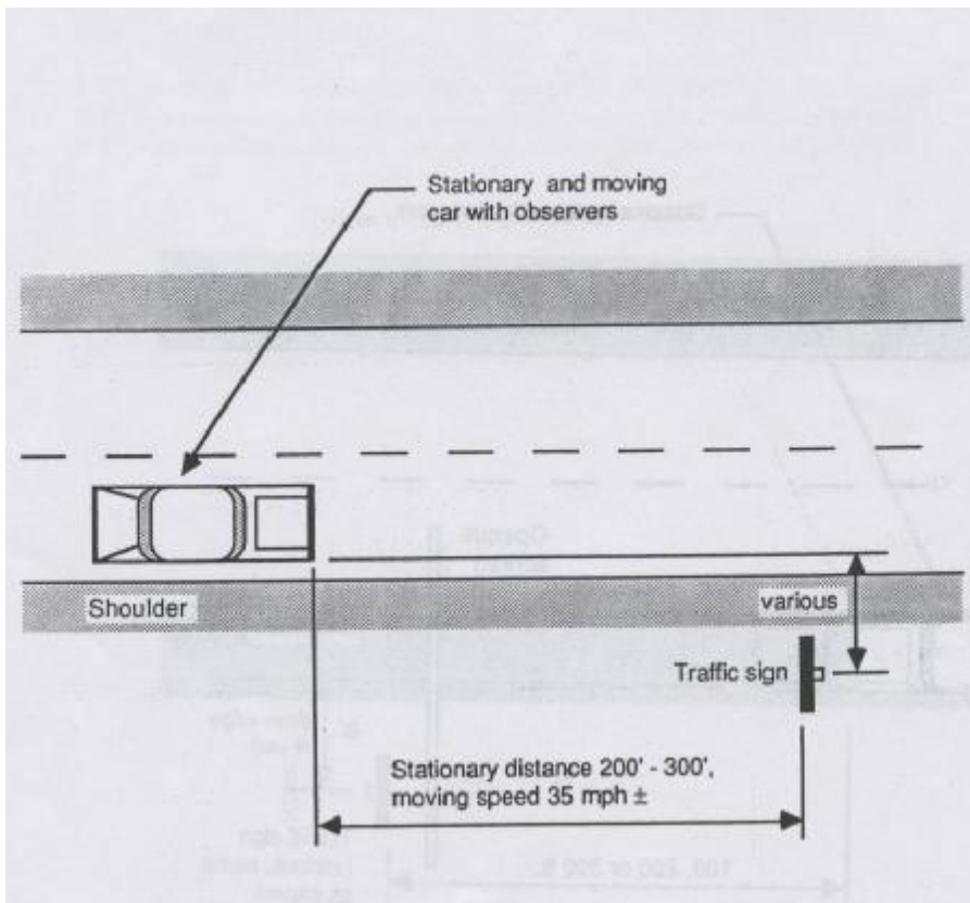
Figure 2.9. Highway Experiment
