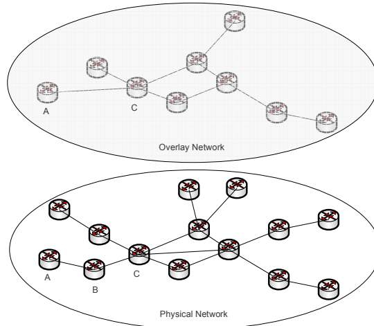
Figure 6.3: Overlay Network
