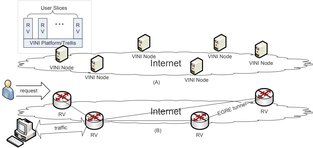
Figure 6.11: VINI
