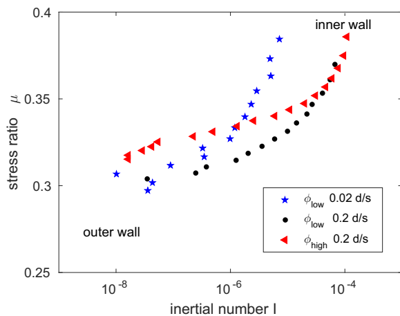
Figure 5. Sample \mu(I) curves for all 3 cases.
