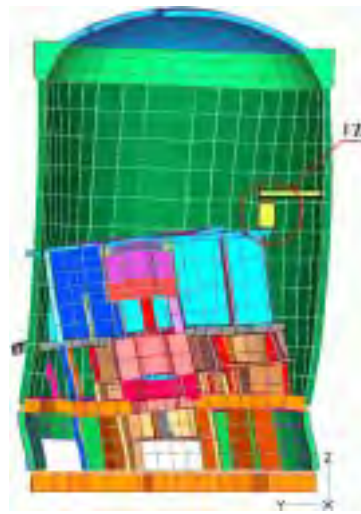
Fig.13 Spatial Model. Mode Shape with Frequency 5.2 Hz and Modal Mass 20%
