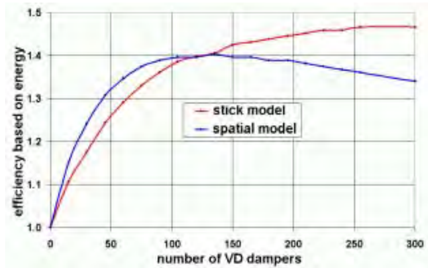
Fig.15 HVD-approach Efficiency Based on Energy
