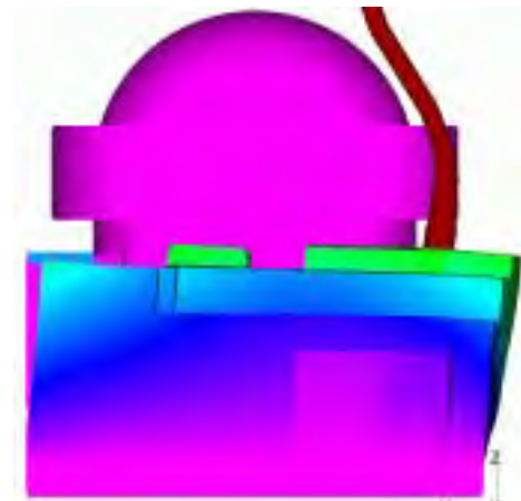
Fig. 29 General Mode Shape of the Special Building (8.66 Hz)
