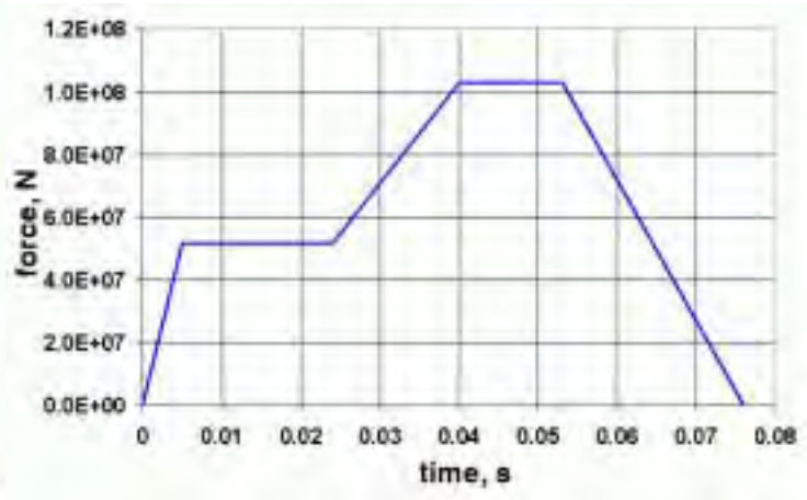
Fig.19 Phantom's Crash Load
