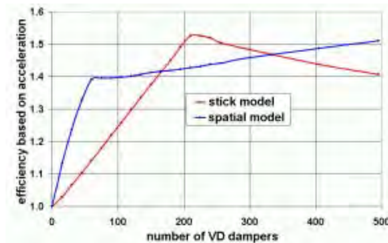
Fig.14 HVD-approach Efficiency Based on Acceleration
