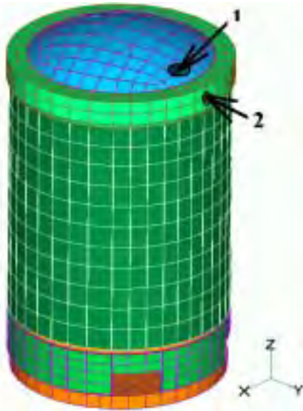
Fig.18 Plane Crash Points
