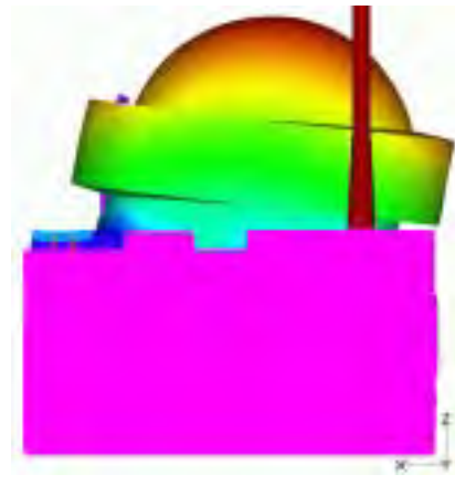
Fig. 27 General Mode Shape of the Reactor Building (3.75 Hz)
