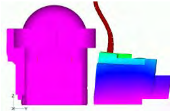
Fig. 28 General Mode Shape of the Special Building (7.66 Hz)
