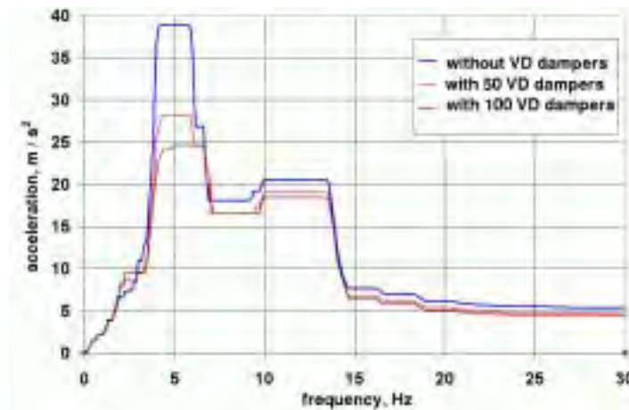
Fig.31 The Seismic Broaden Response Spectra for the Roof of the Special Building (Damping 2%)
